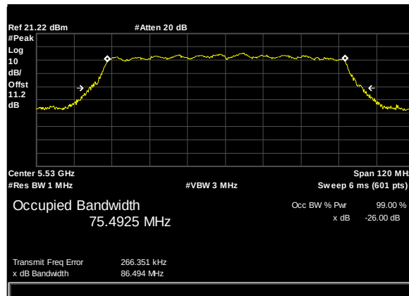
Plot 36. 26 dB Occupied Bandwidth, BW 80M, Ch 5530M, AC Mode ANT 0
