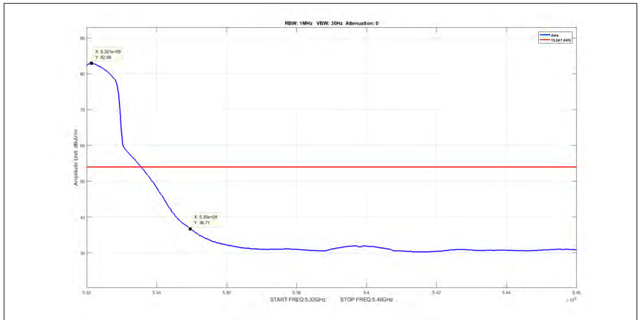
Plot 123. Undesirable Emissions, Average Band Edge Spurious, BW 20M, Ch 5320M, N Mode ANT 0 (worst-case)
