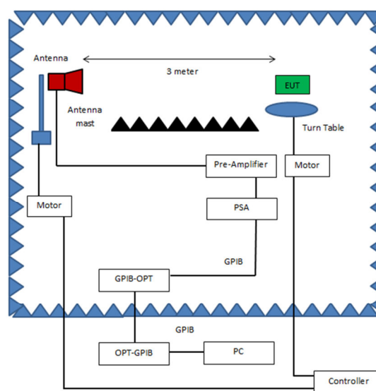
Radiated Emissions, Above 1GHz, Test Setup
