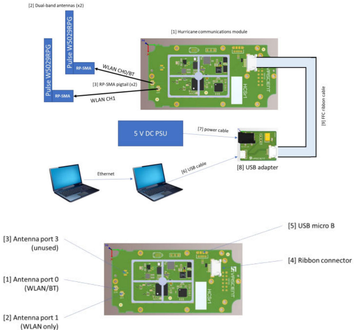
Block Diagram
