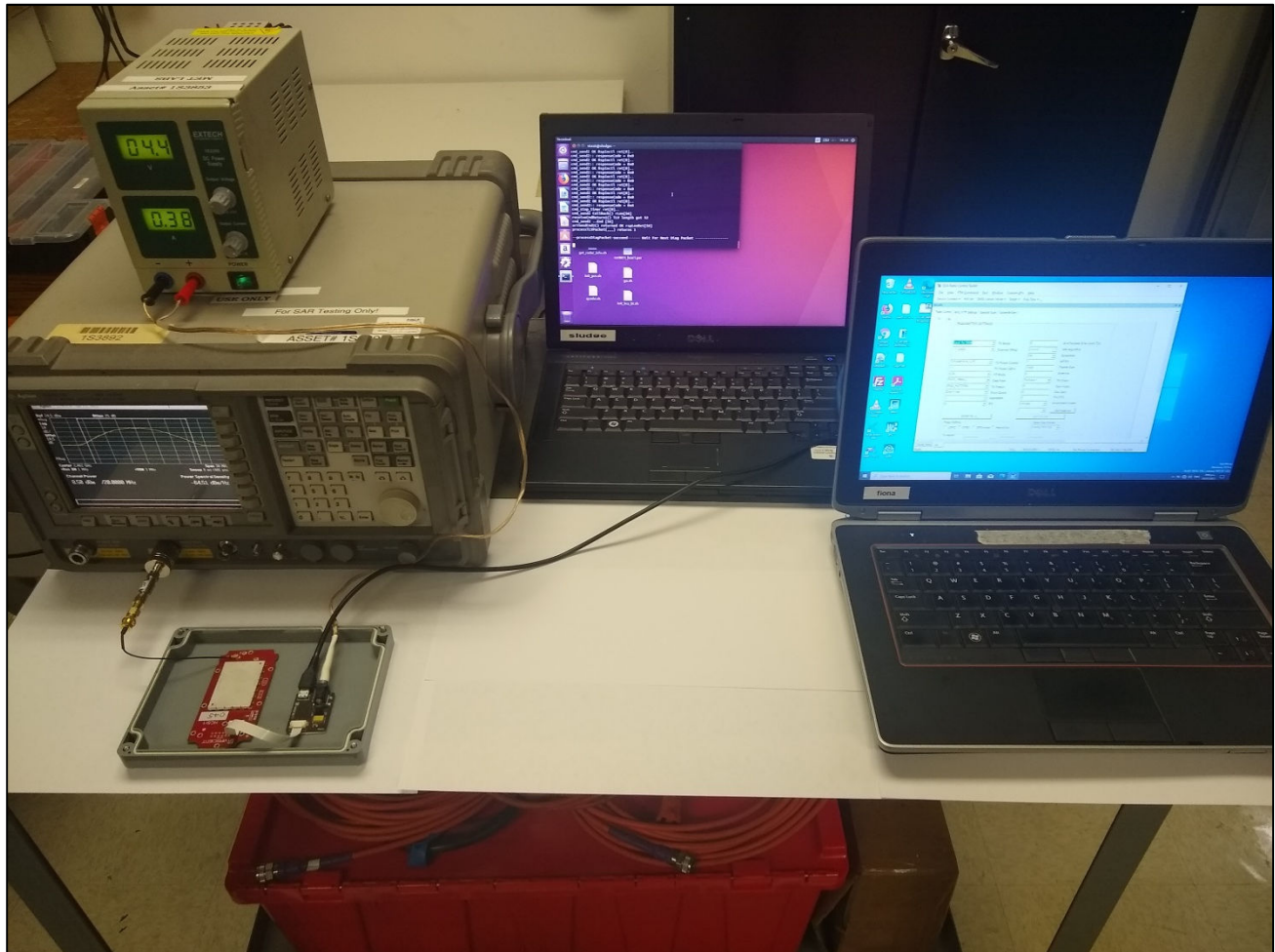
Conducted Measurement Test Setup
