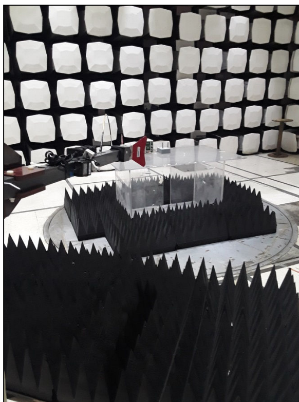
Photograph 2. Radiated Spurious Emissions, Above 1 GHz, Test Setup
