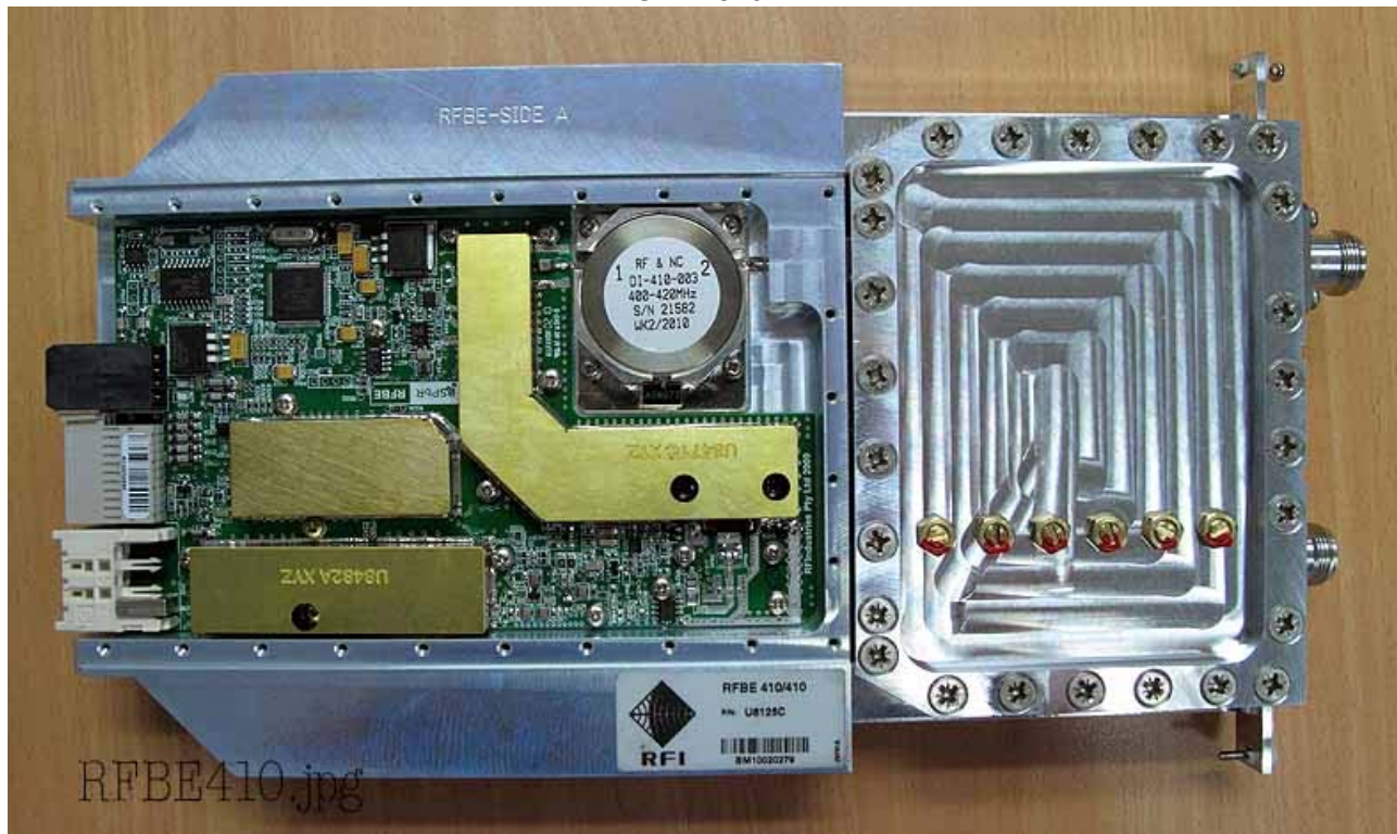
PCB Front
