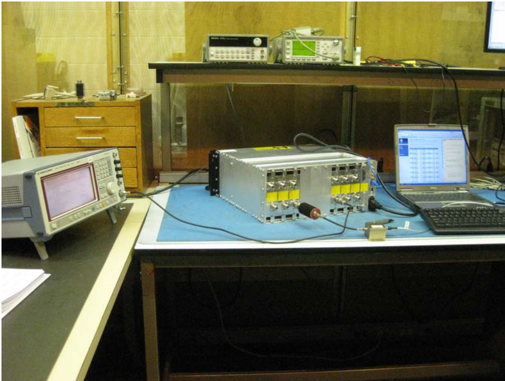
Conducted #2
