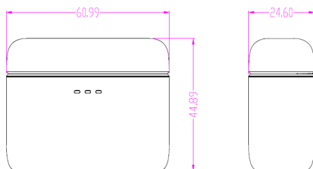
Charging box
