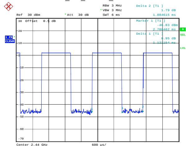
BLE_2M_Middle_Channel
