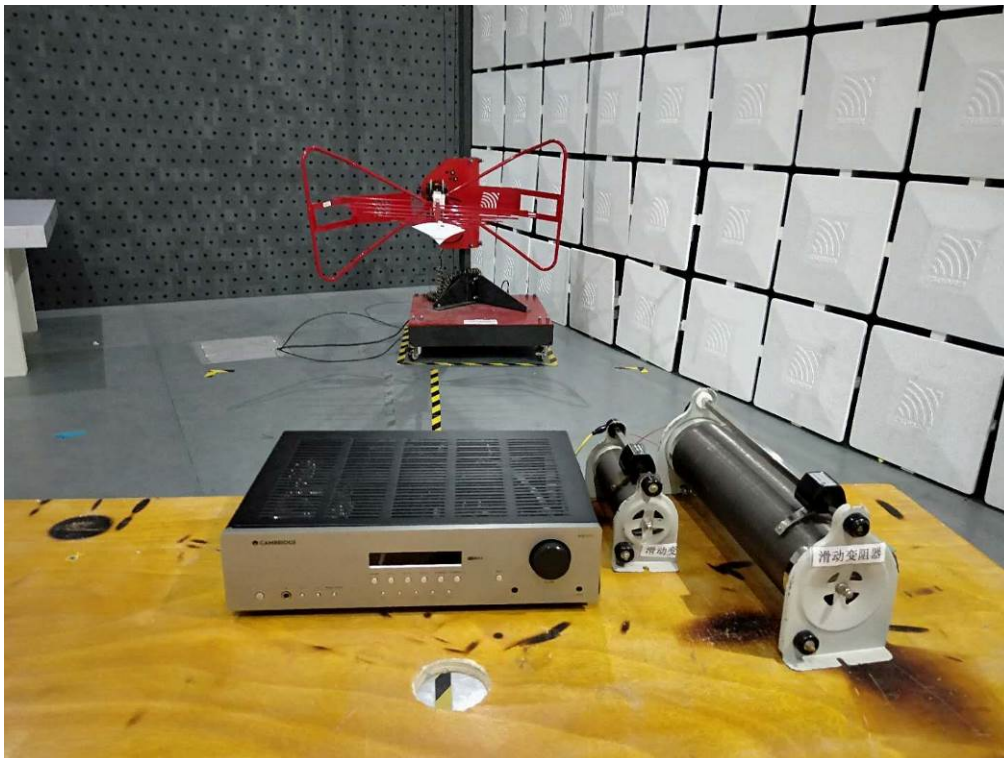
Radiated Emissions, 30MHz to 1GHz Test Setup
