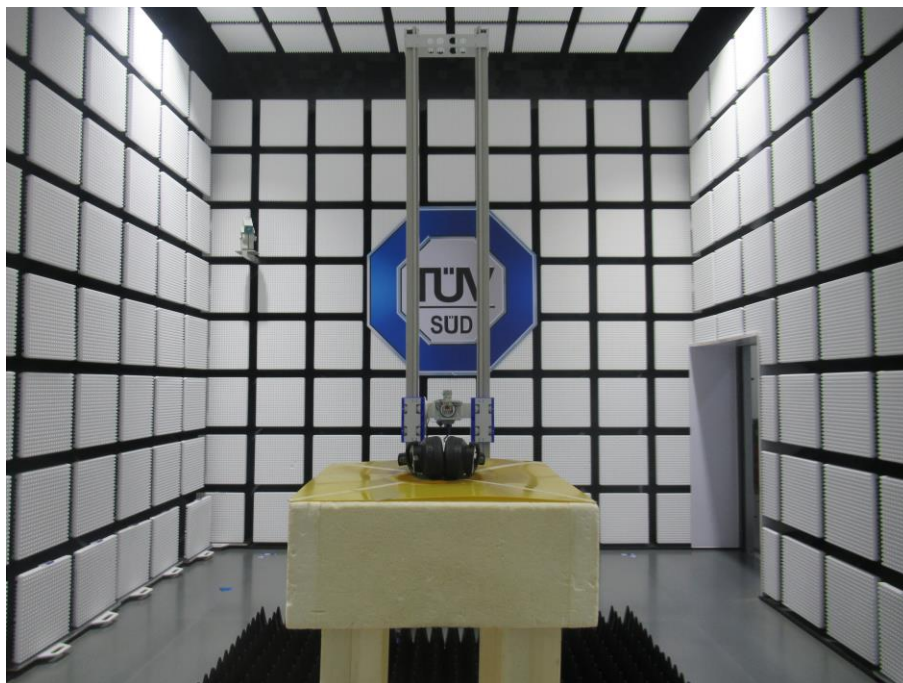
Radiated Emission Test above 18GHz
