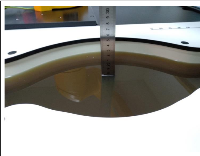
Head Liquid depth in the Twin-SAM Phantom
