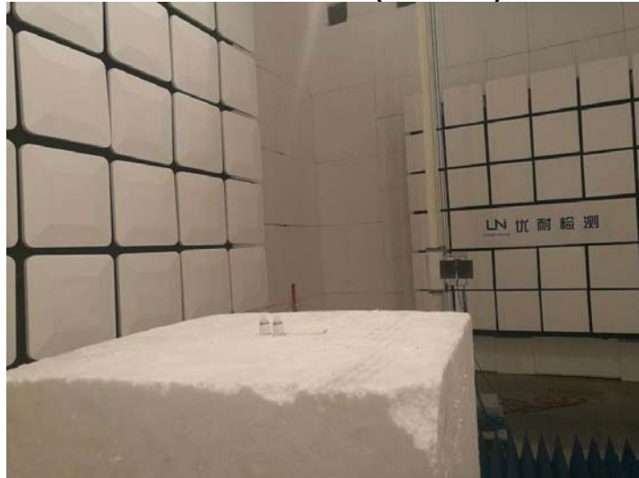
Radiated Emission (Above 1G)
