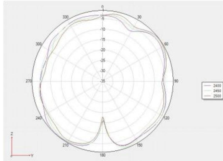
Phi 90 2D
