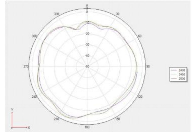
Theta 90 2D
