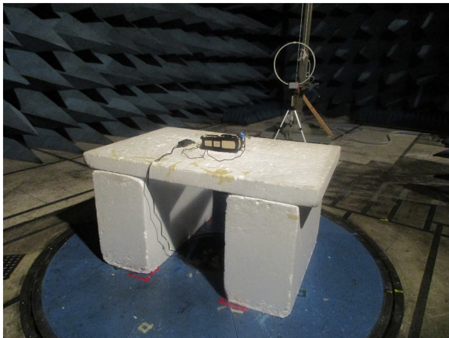
Figure 6: Back – Radiated Emissions
