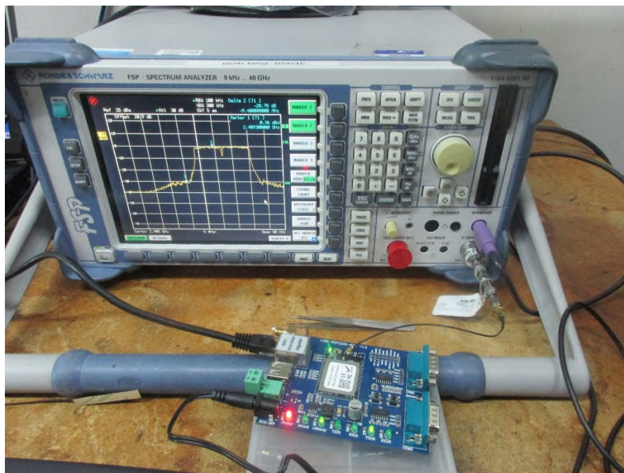
Figure 9: RF Conducted
