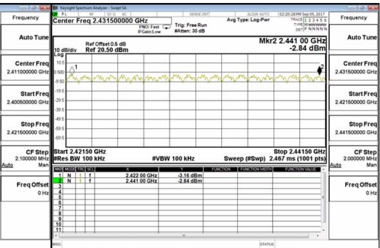
2422-2441MHz
