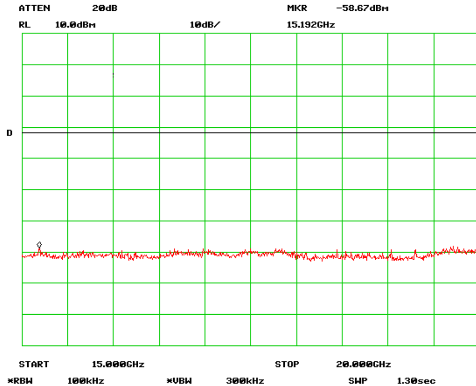
Antenna Port Emission High-5 Channel (802.11g)
