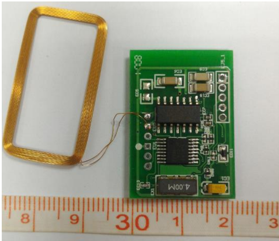
Low Frequency PCA with Antenna – Bottom View
