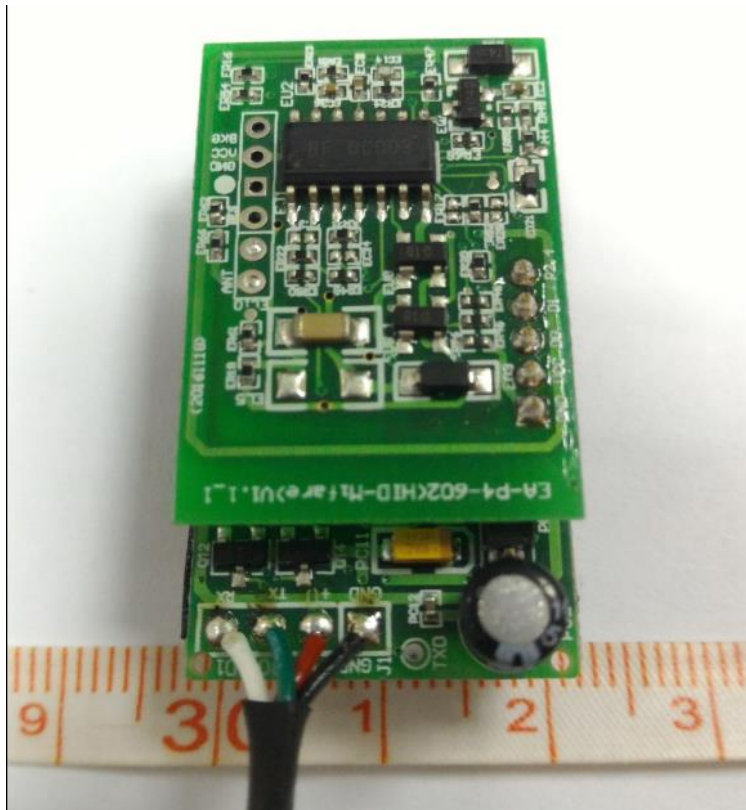
Full Assembly – Top View
