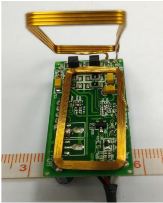
Full Assembly – Bottom View (Shield Removed)
