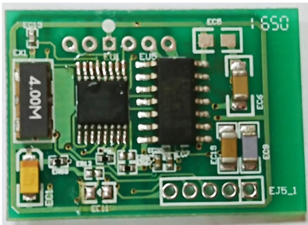
Low Frequency PCA – Bottom View
