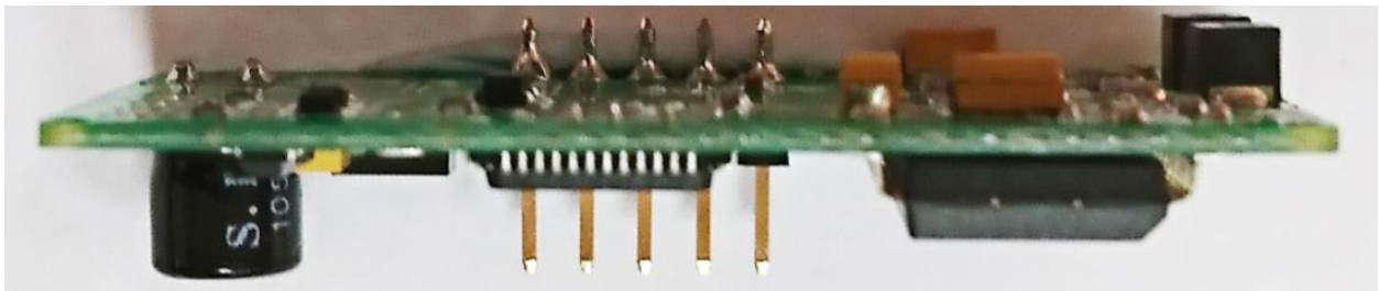
High Frequency PCA – Side View
