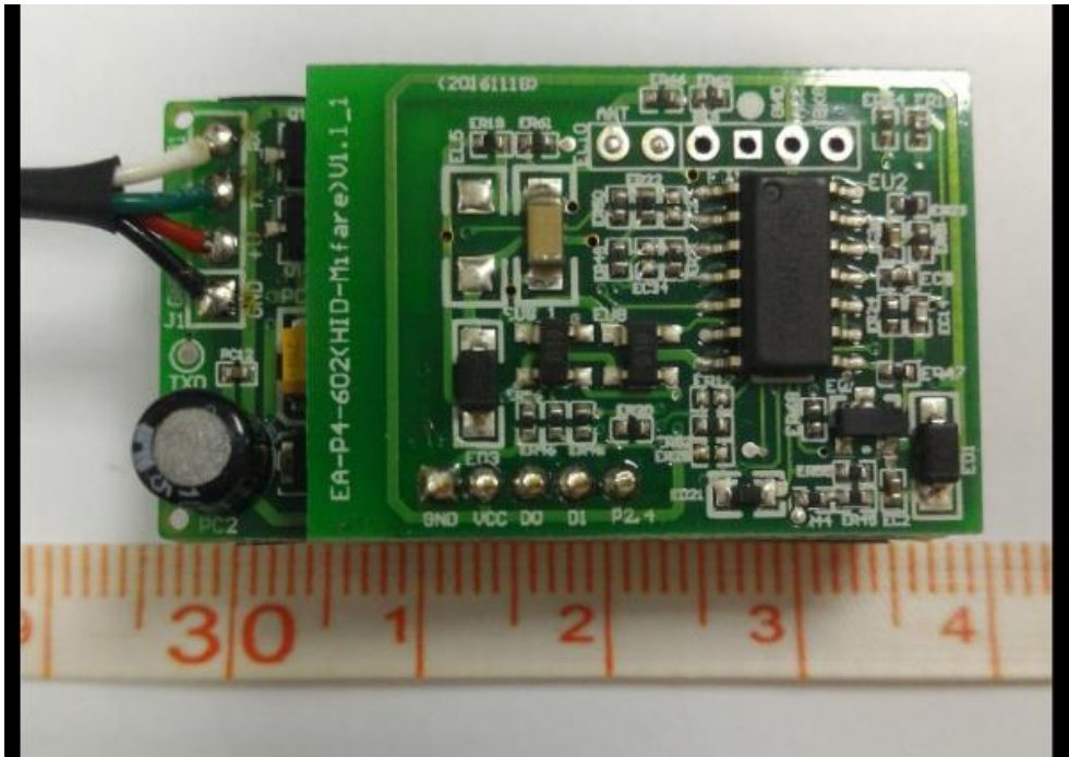
Full Assembly – Top View
