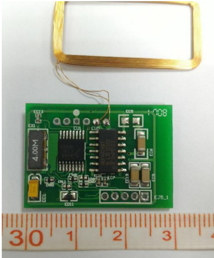
Low Frequency PCA with Antenna – Bottom View
