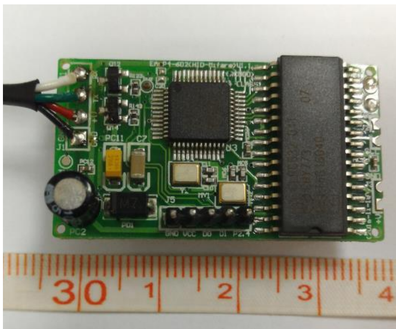
High Frequency PCA – Top View
