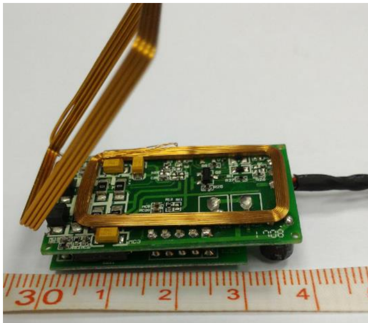
Full Assembly – Bottom View (Shield Removed)
