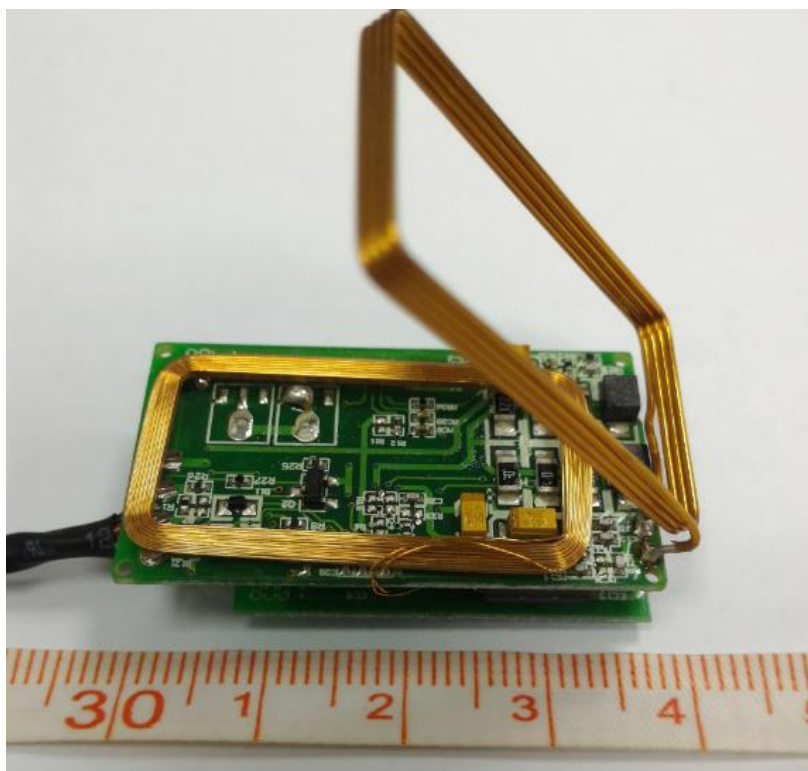
Full Assembly – Bottom View (Shield Removed)
