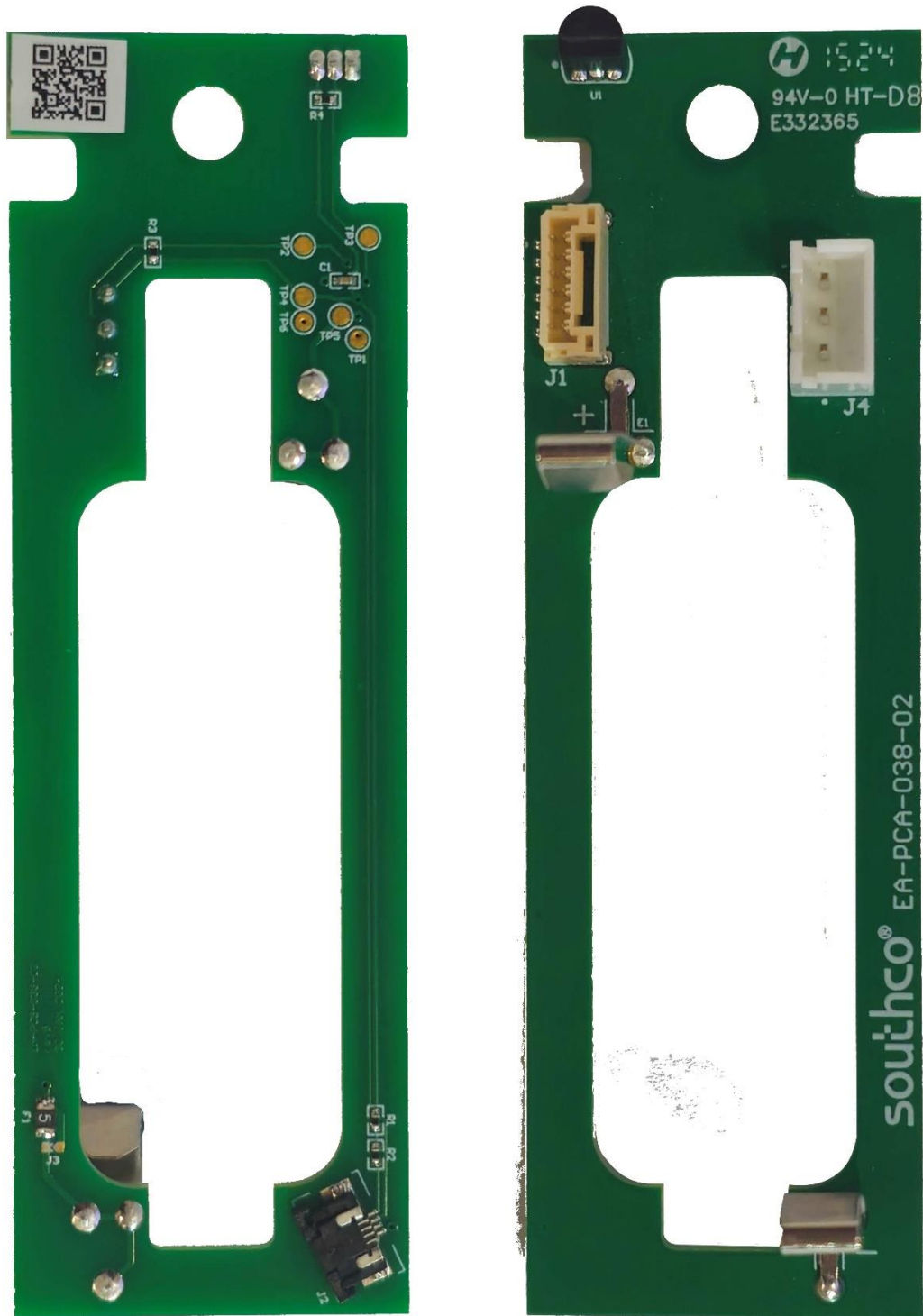
Picture 7: EA-PCA-038-02 (Both Sides)
