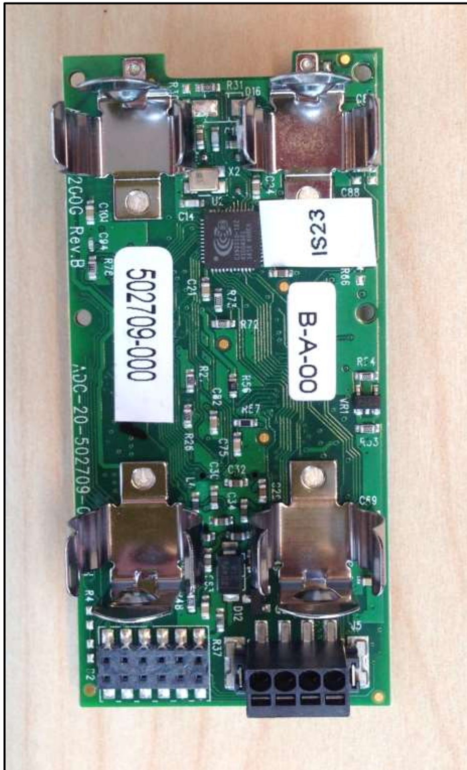
Photograph 11: PCB Back
