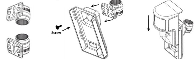
Mounting Arm Orientation Attach Mounting Arm to Sensor-Back Attach Sensor to Sensor-Back (Top: Teeth Up, Bottom: Teeth Down)
