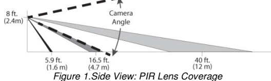
Figure 1. Side View: PIR Lens Coverage
