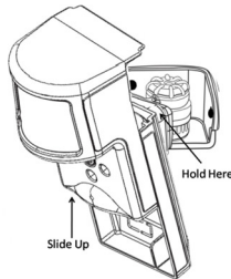
Figure 4. Removing Sensor for Battery Replacement
