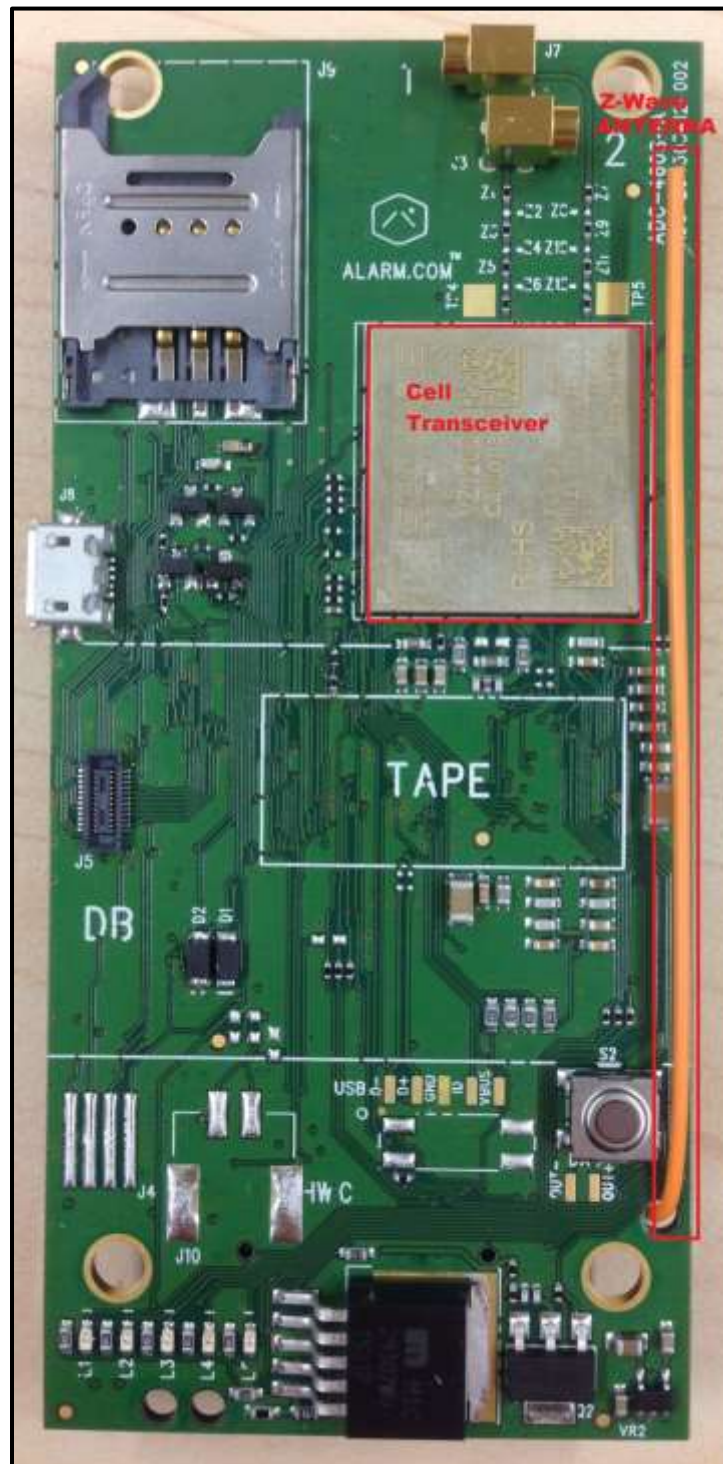
Photograph 17: PCB Top - Labeled
