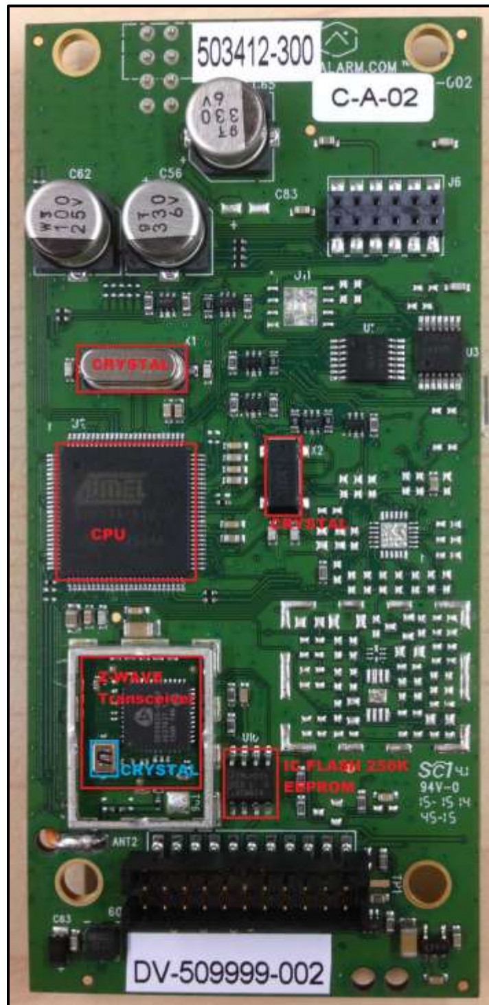
Photograph 21: PCB Bottom without Shield, Labeled
