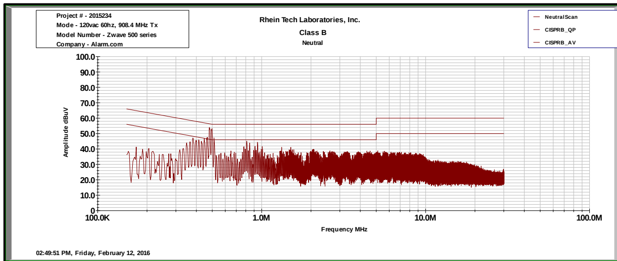
Plot 4-1: Conducted Emissions Transmit - Neutral Side
