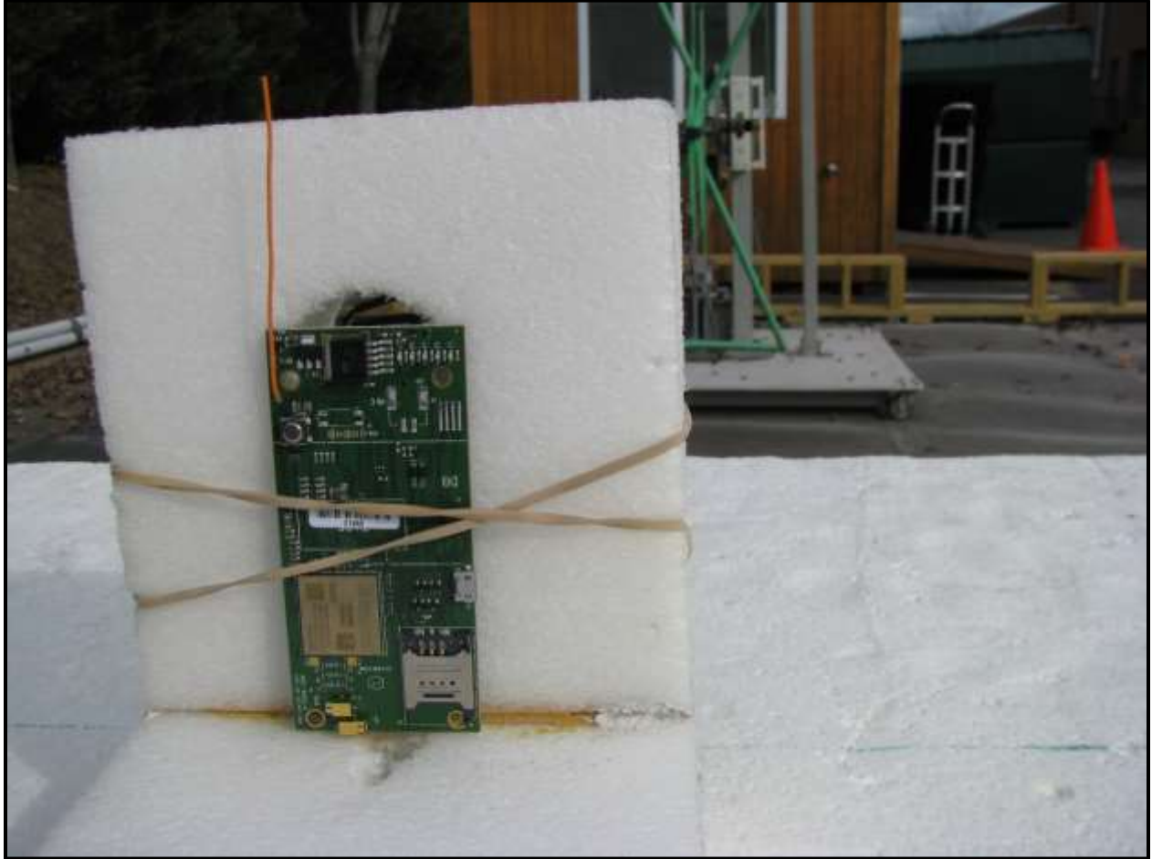
Photograph 5: Radiated Emissions Testing
