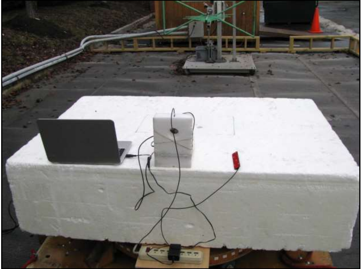
Photograph 7: Radiated Emissions, Digital Unintentional Emissions
