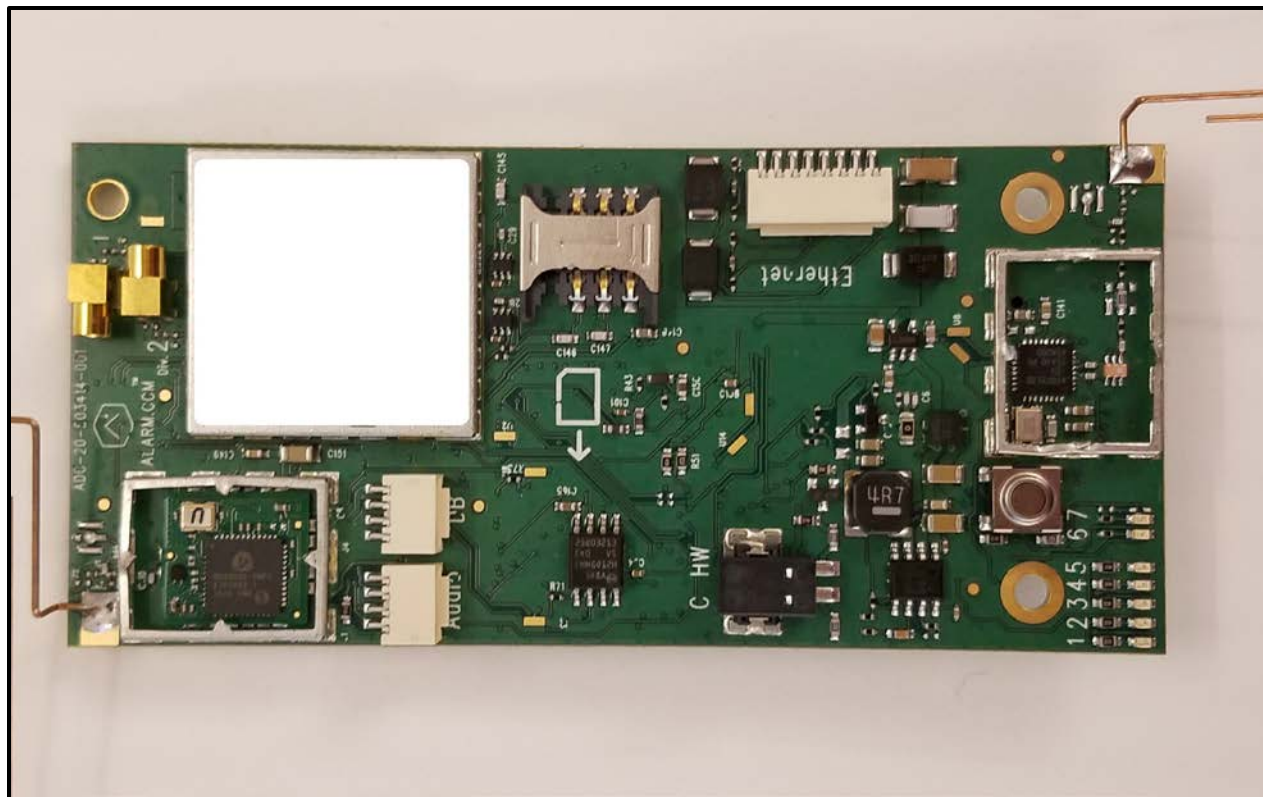
Photograph 12: Module Top View – No Shields
