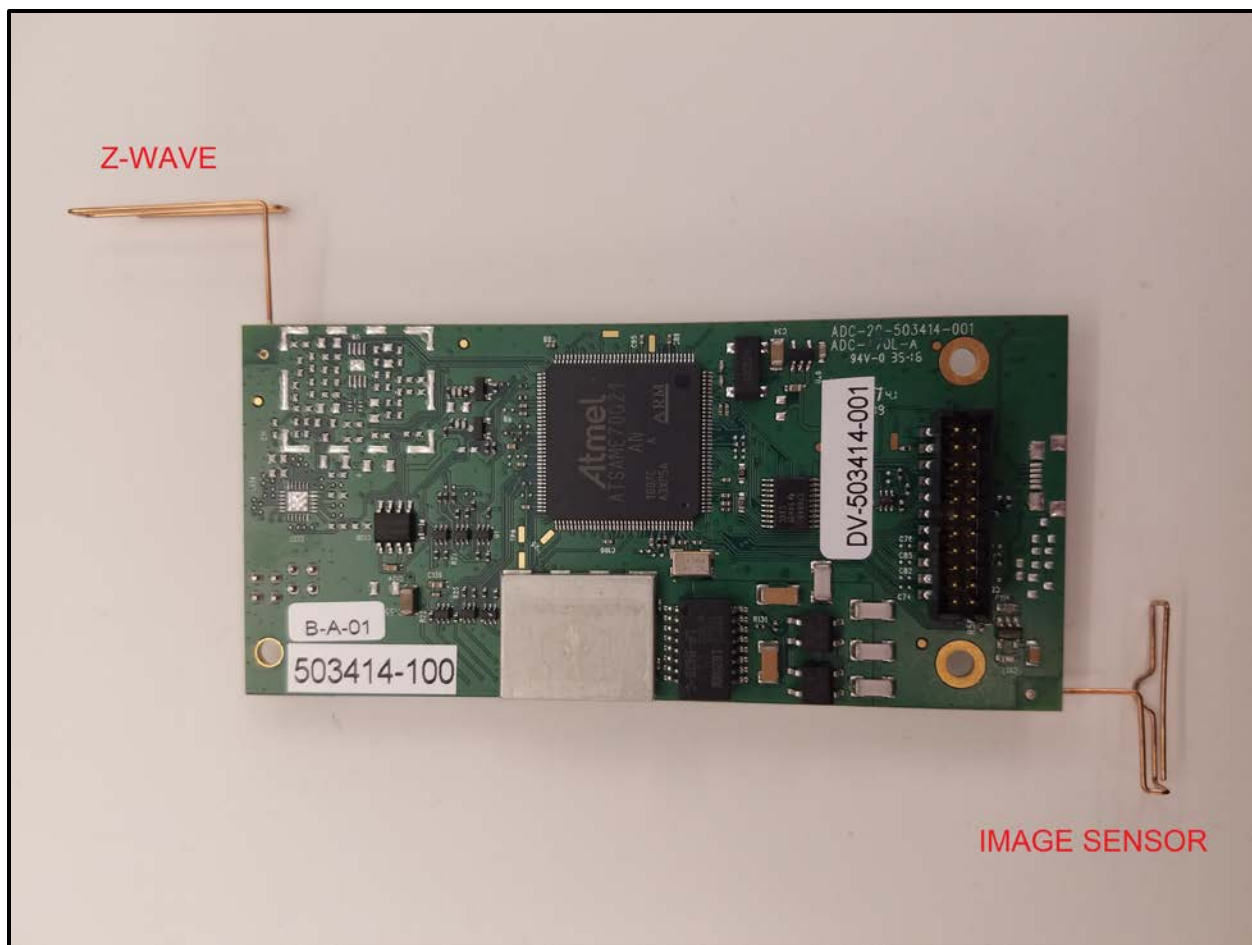
Photograph 11: Module Bottom View
