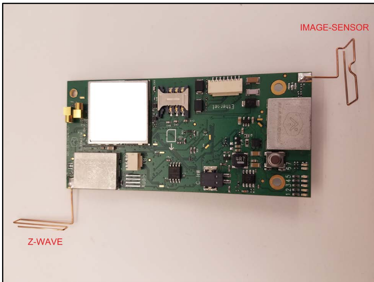
Photograph 10: Module Top View
