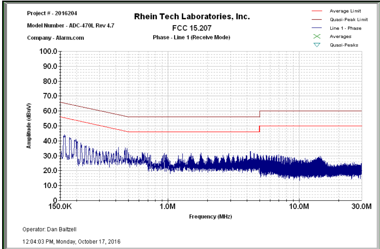
Plot 9-1: Conducted Emissions - Phase - Receive Mode
