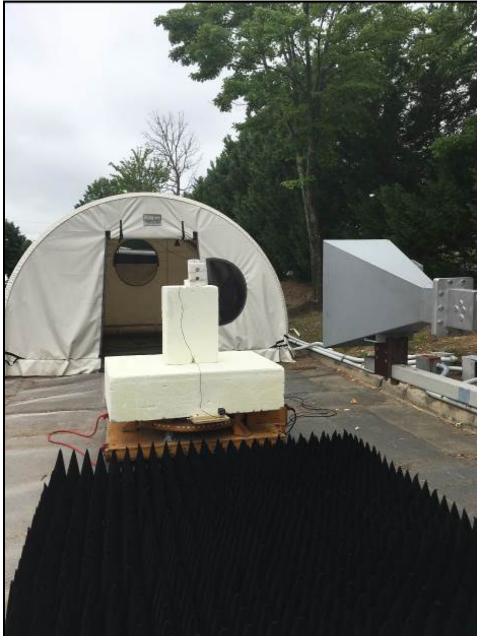
Photograph 4: Radiated Emissions Testing – Back View (Spurious Emissions, >1 GHz)
