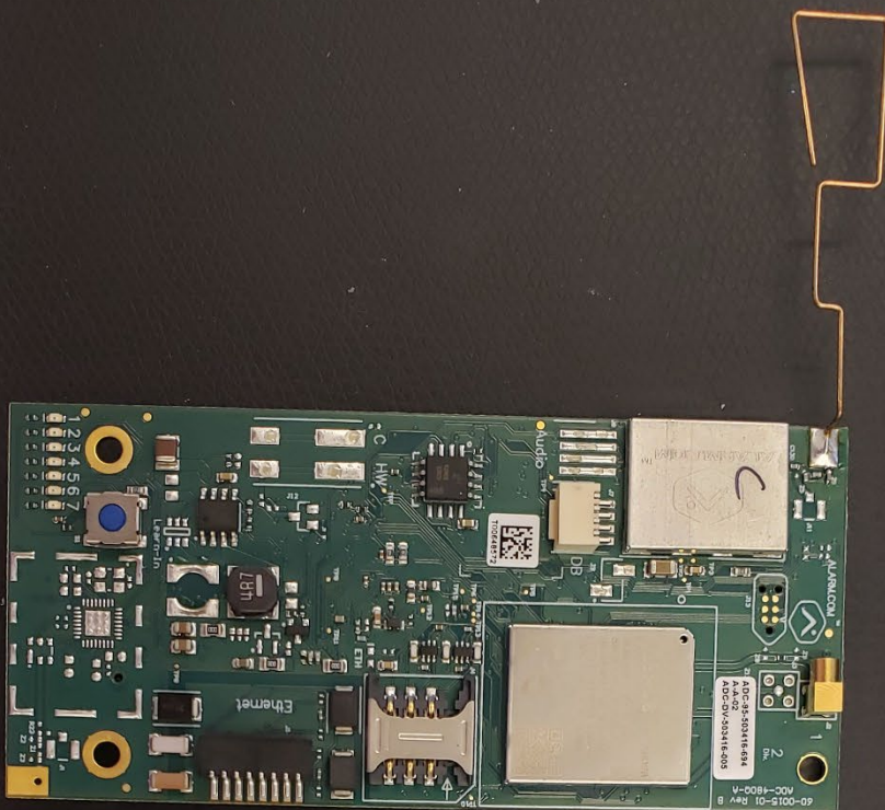
Concord Z-Wave Antenna
