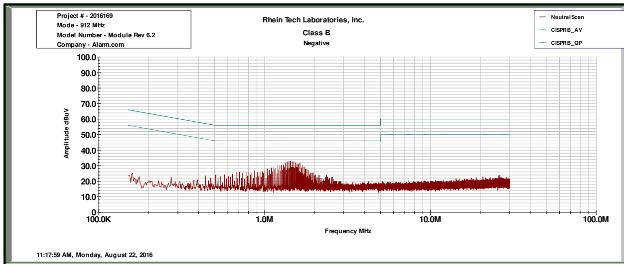
Plot 9-4: Conducted Emissions - VDC Return - Transmit
