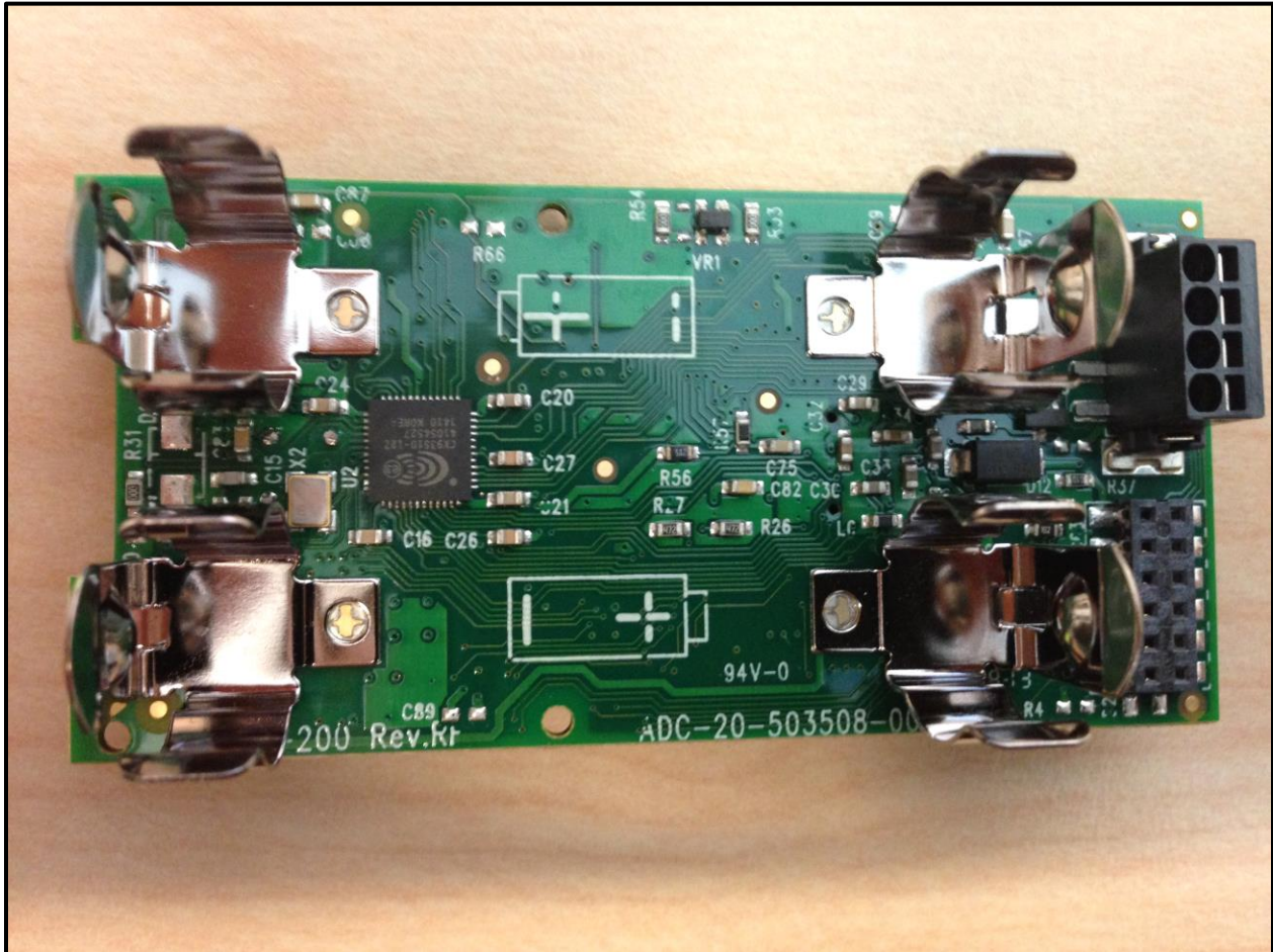
Photograph 6: PCB Side 1
