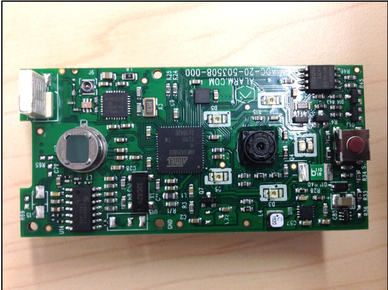
Photograph 7: PCB Side 2
