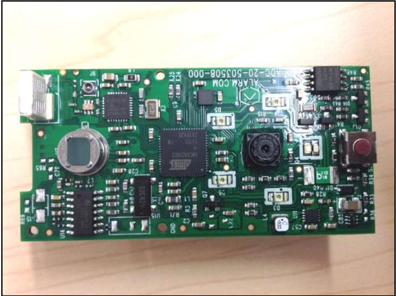
Photograph 8: PCB Side 2
