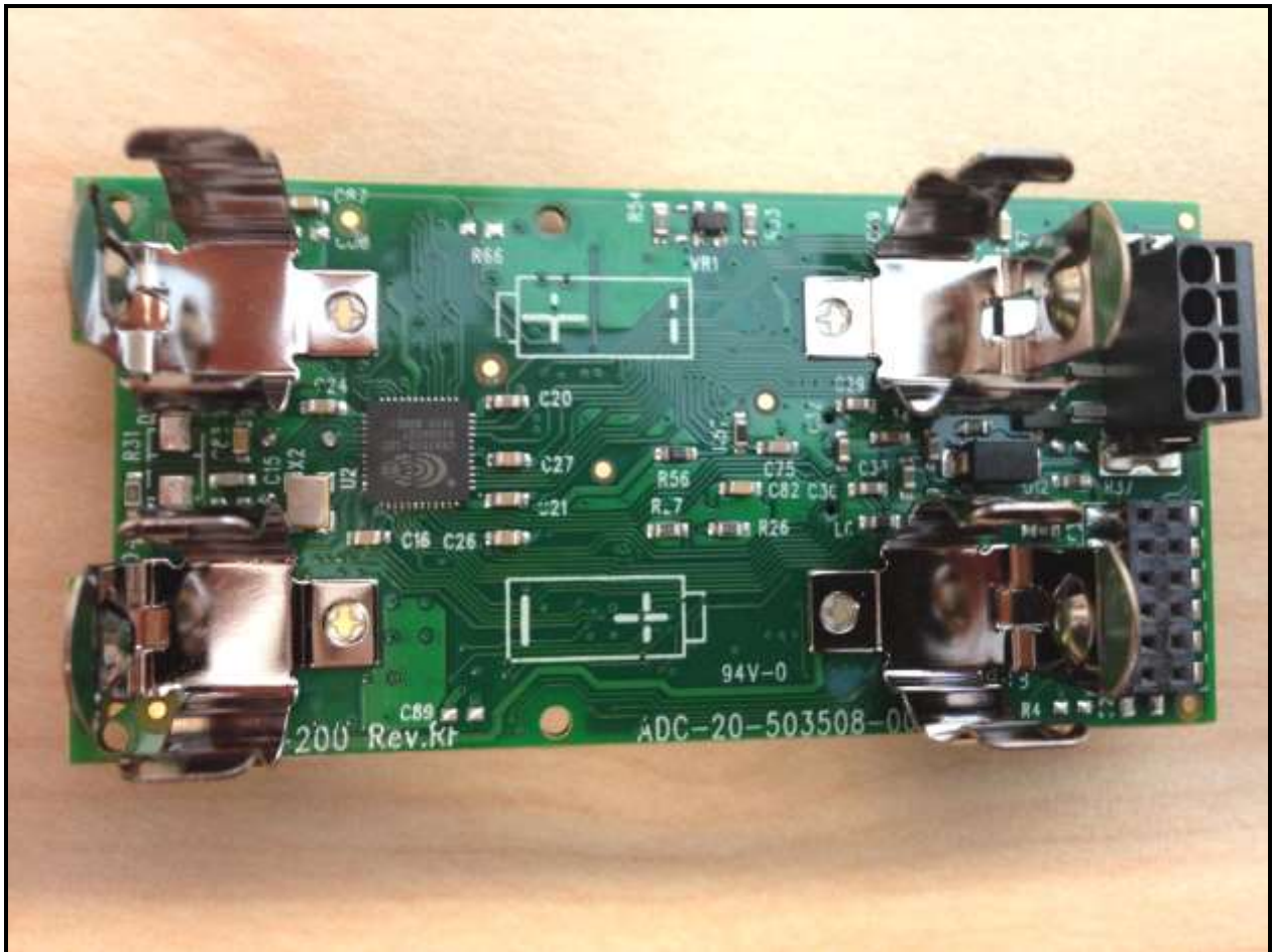
Photograph 7: PCB Side 1
