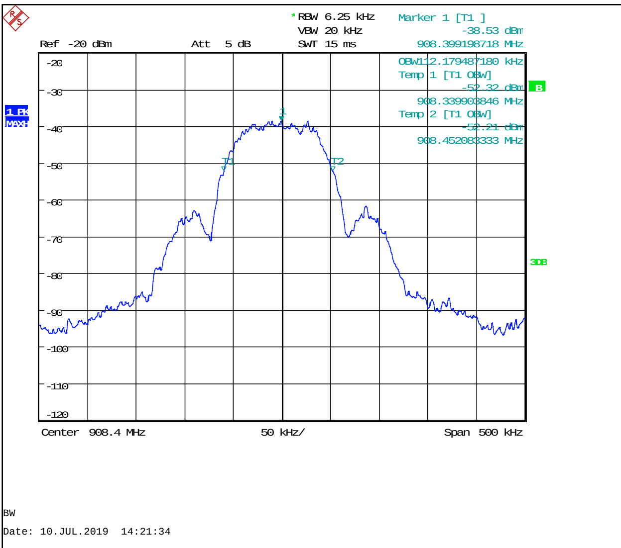
Plot 5-1: 99% Bandwidth – 908.4 MHz
