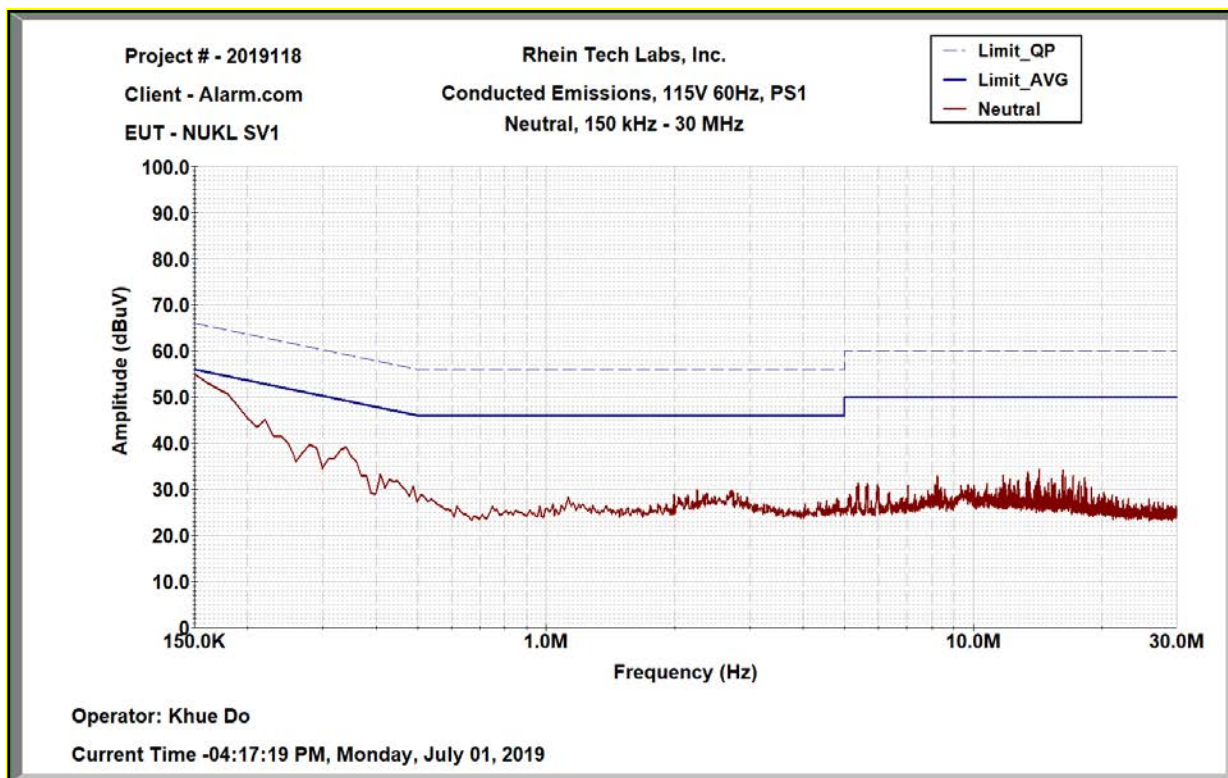
Plot 4-8: Conducted Emissions – Neutral - SVL LTE; Power Supply #1
