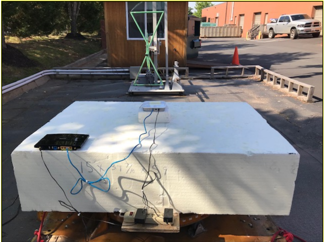
Photograph 2: Radiated Emissions Testing – Back View (Digital Emissions, <1 GHz)
