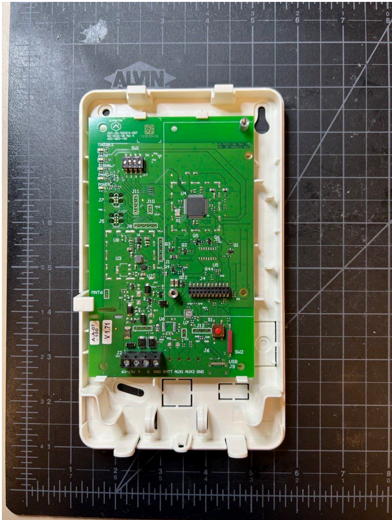
ADC-SEM-300 – Photo13 – Top View of Bottom PCB in Chassis after Top PCB Removed
