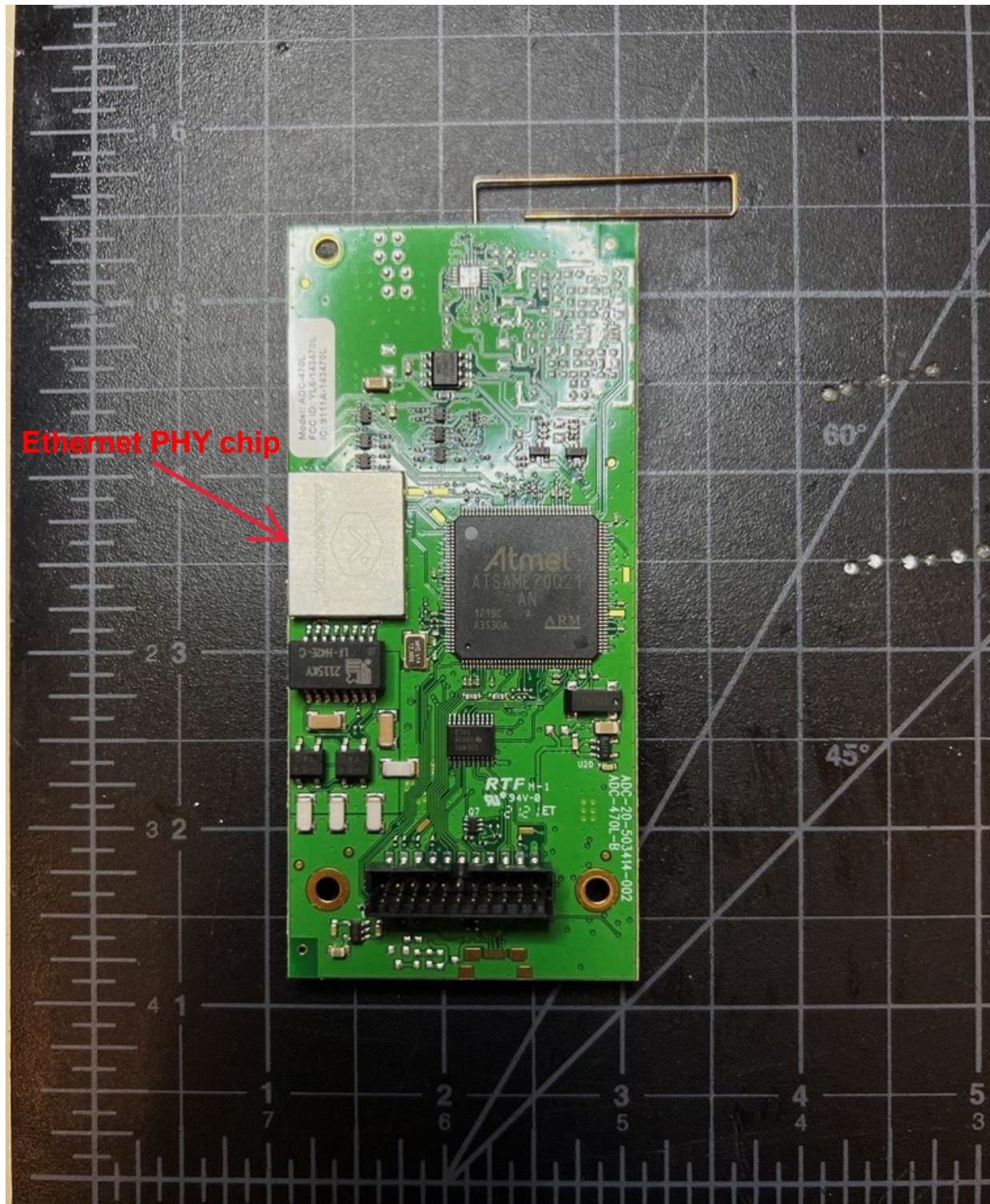
ADC-SEM-300 – Photo 8 – Top PCB – Bottom View
