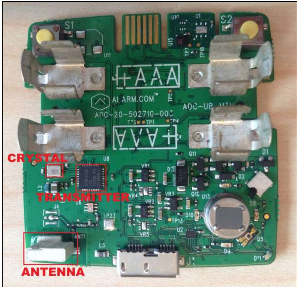
Photograph 16: PCB – Top
