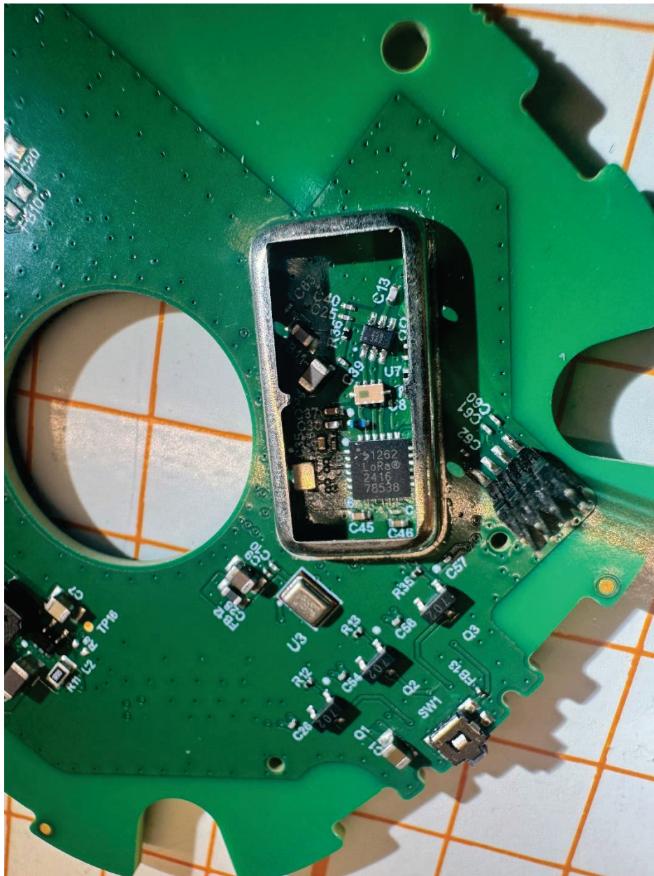
LoRa Chip Underneath RF shield of IRLED board
