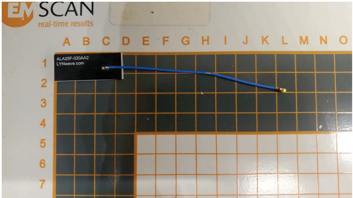
Lynwave Antenna (ALA25F-020AA2-00) [LoRa option 2]
