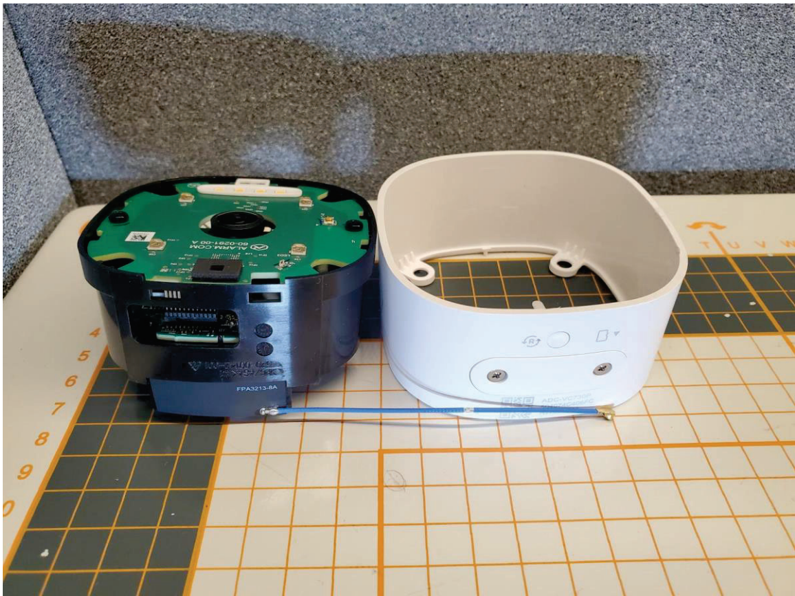
Inpaq Antenna (RFFPA321309IMRB402) [LoRa option 1]
