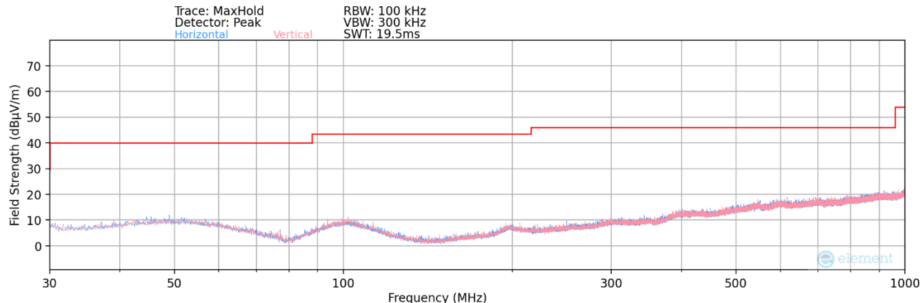
Plot 7-32. Radiated Spurious Plot below 1GHz
