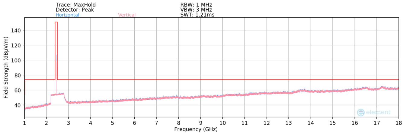
Plot 7-29. Radiated Measurements Plot
