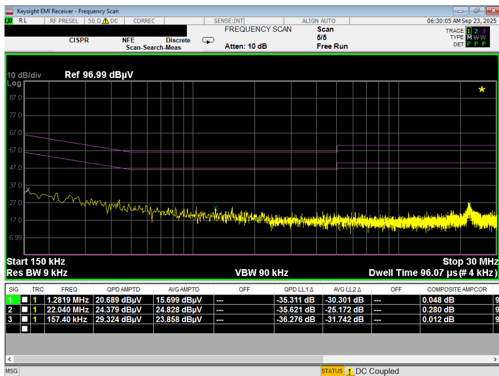
Plot 7-34. Line Conducted Plot with Bluetooth LE (N)
