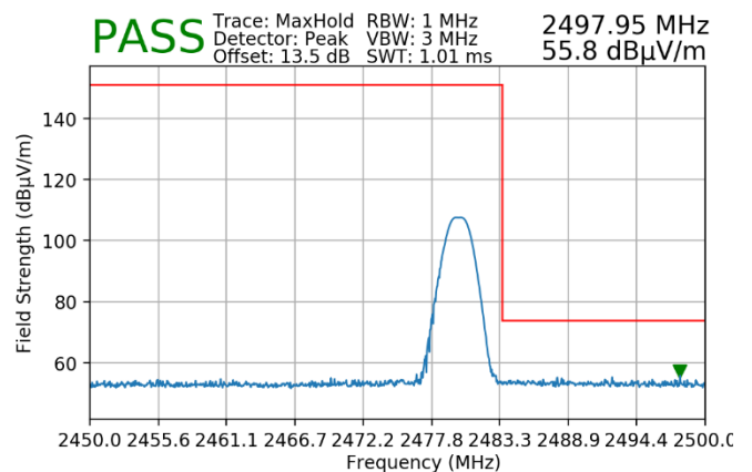
Plot 7-31. Radiated Restricted Upper Band Edge Measurement (Peak)
