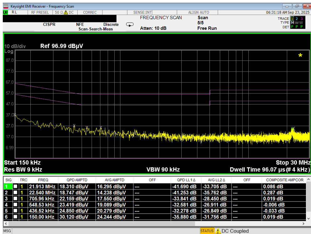
Plot 7-33. Line Conducted Plot with Bluetooth LE (L1)
