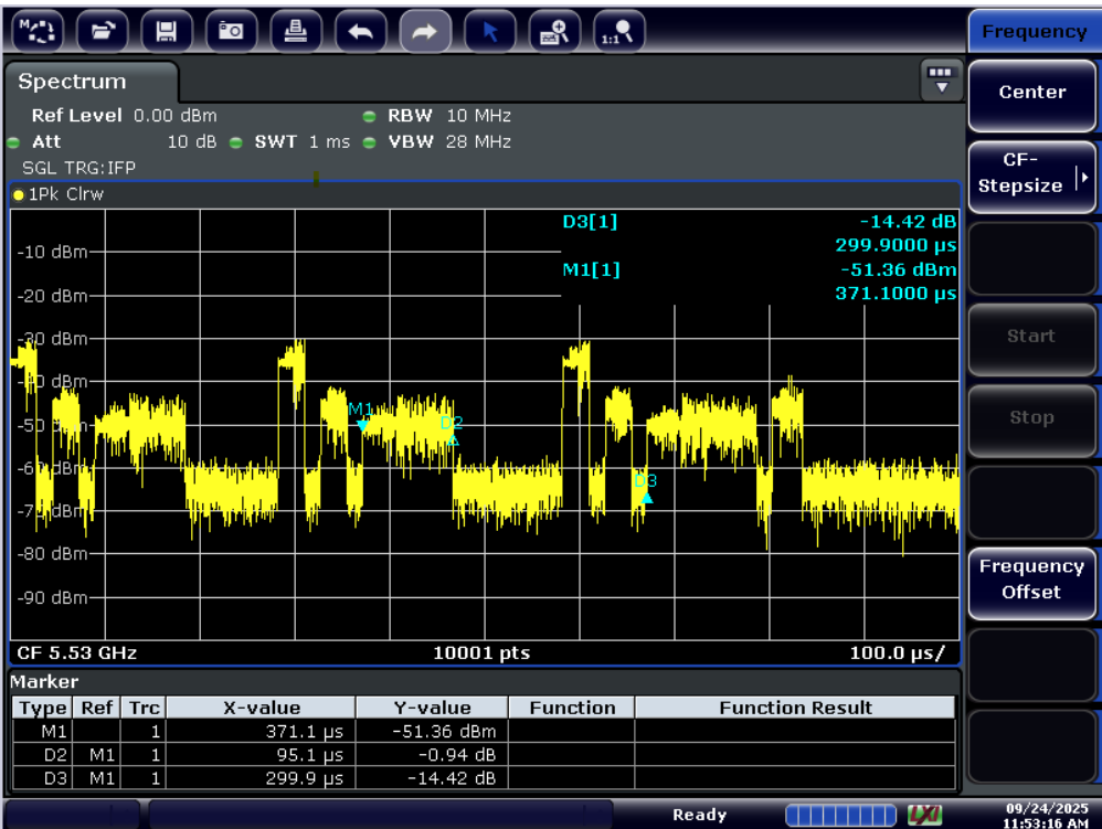
Figure 9-2. Band 2C Period
