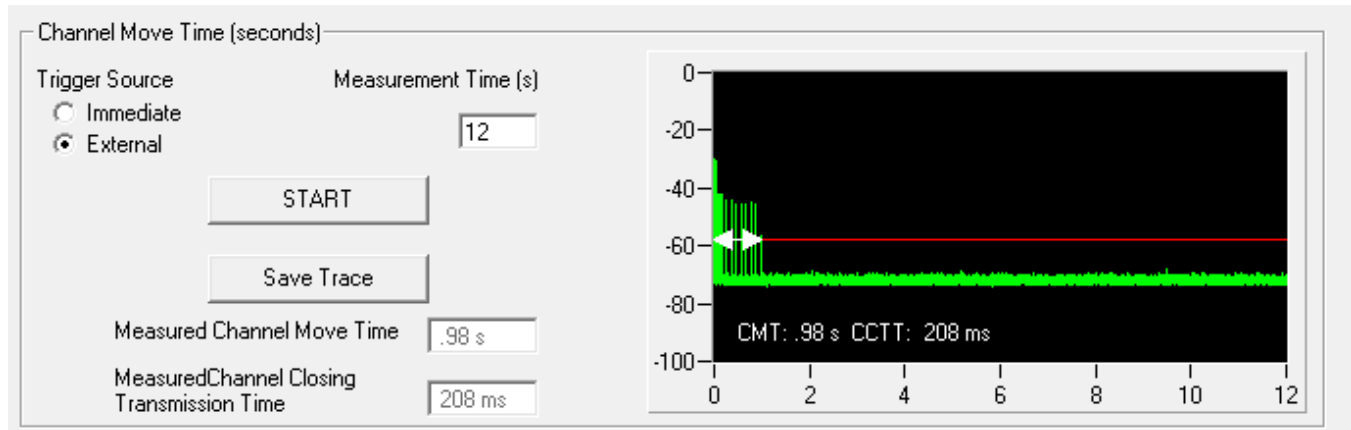
Figure 9-3. Band 2A CMT and CCTT
