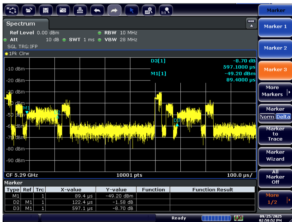
Figure 9-1. Band 2A Period
