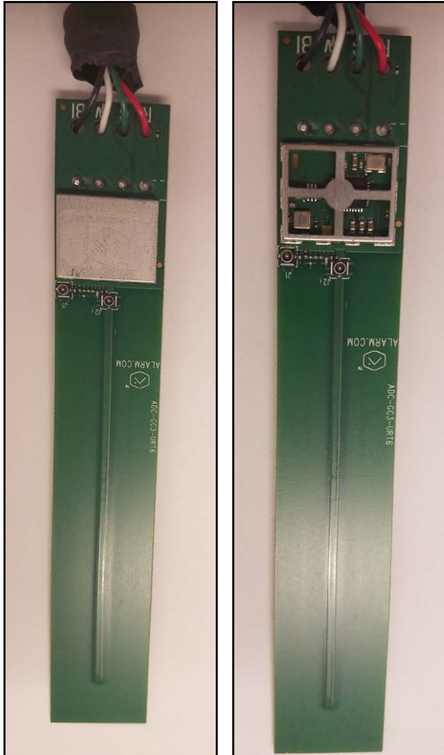
Photograph 12: Bottom View with Shield and Bottom View without Shield
