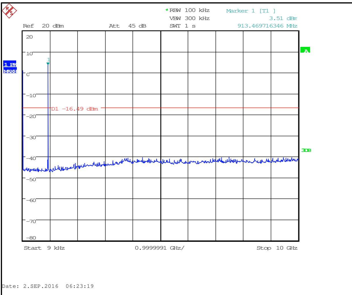
Plot 5-1: Antenna Conducted Spurious Emissions – 912 MHz
