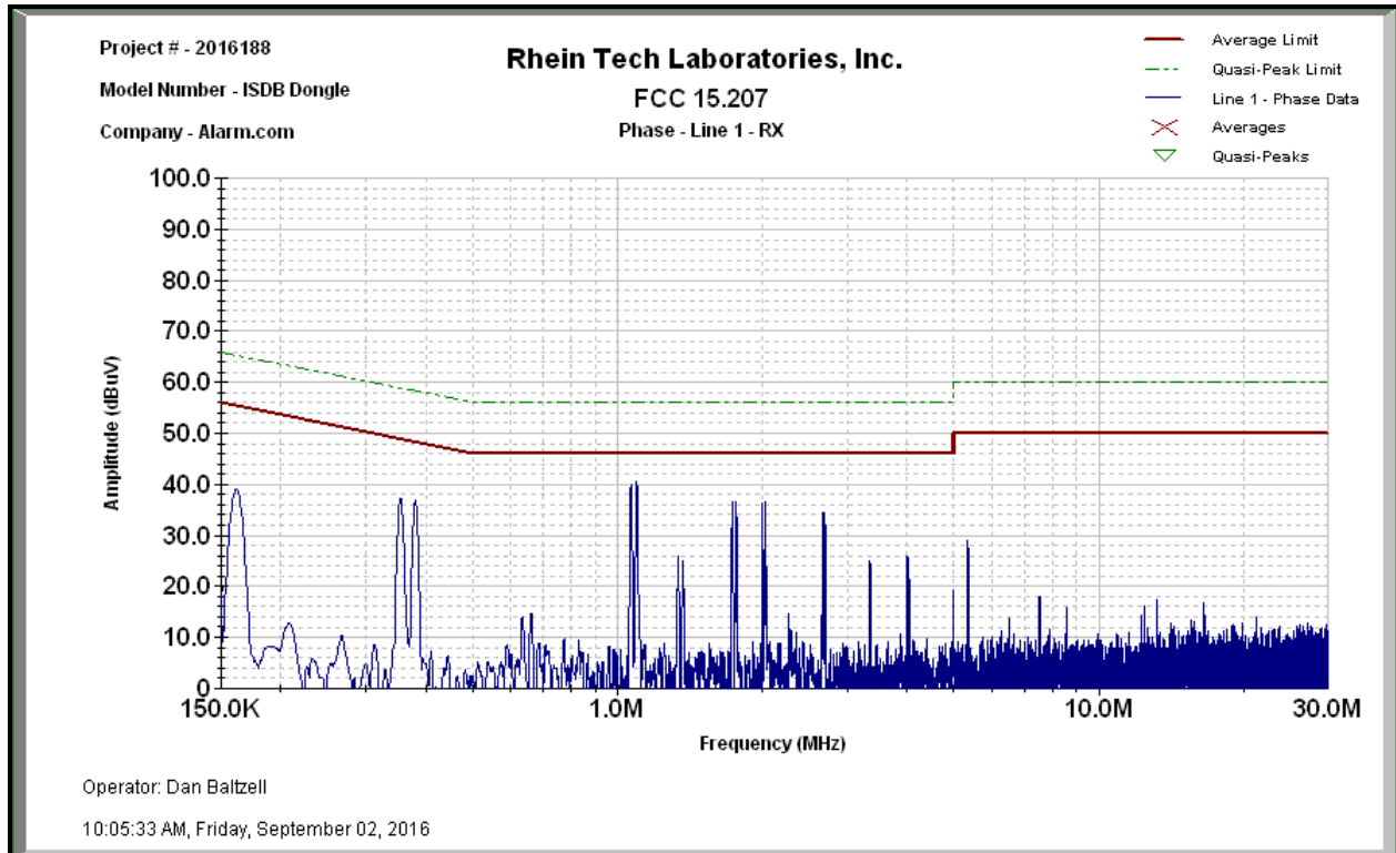
Plot 9-1: Conducted Emissions- Phase - Receive Mode
