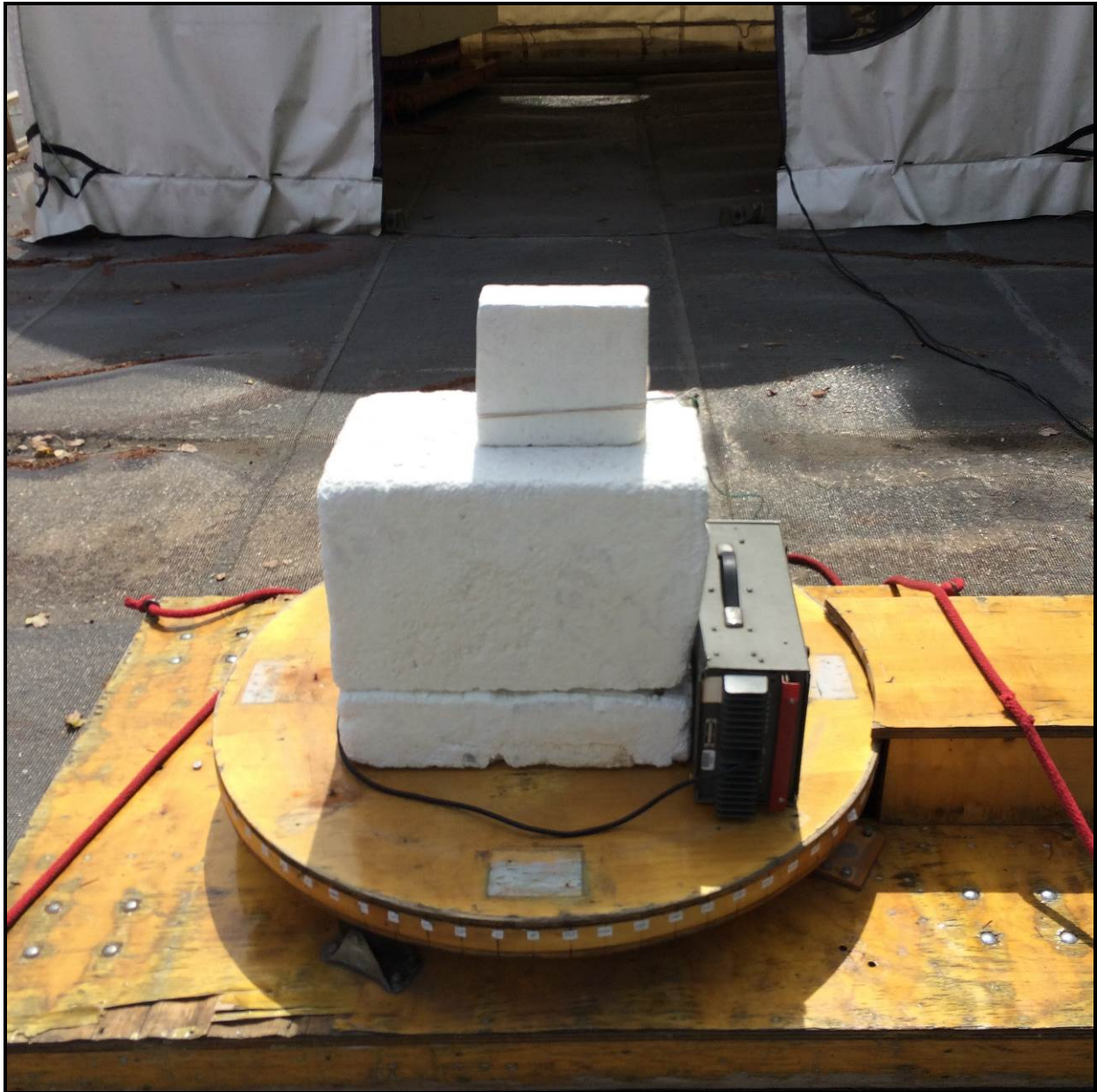
Photograph 4: Radiated Emissions Testing – Back View (Digital Emissions, <1 GHz)
