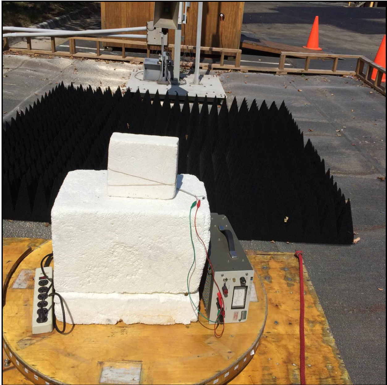
Photograph 6: Radiated Emissions Testing – Back View (Spurious Emissions, >1 GHz)
