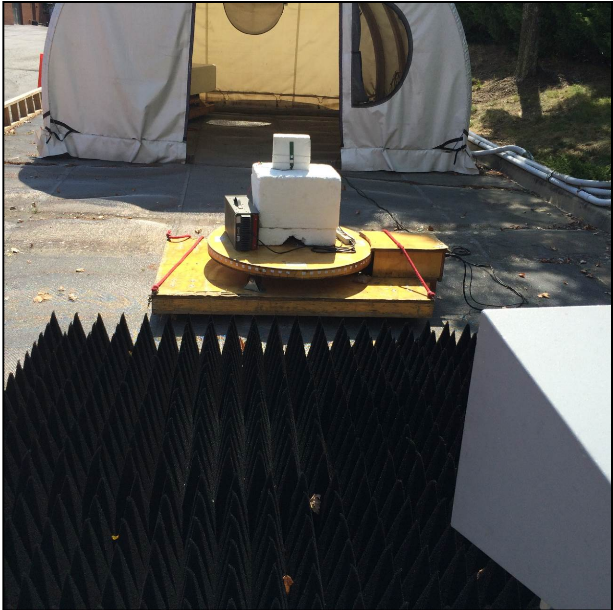
Photograph 5: Radiated Emissions Testing – Front View (Spurious Emissions, >1 GHz)
