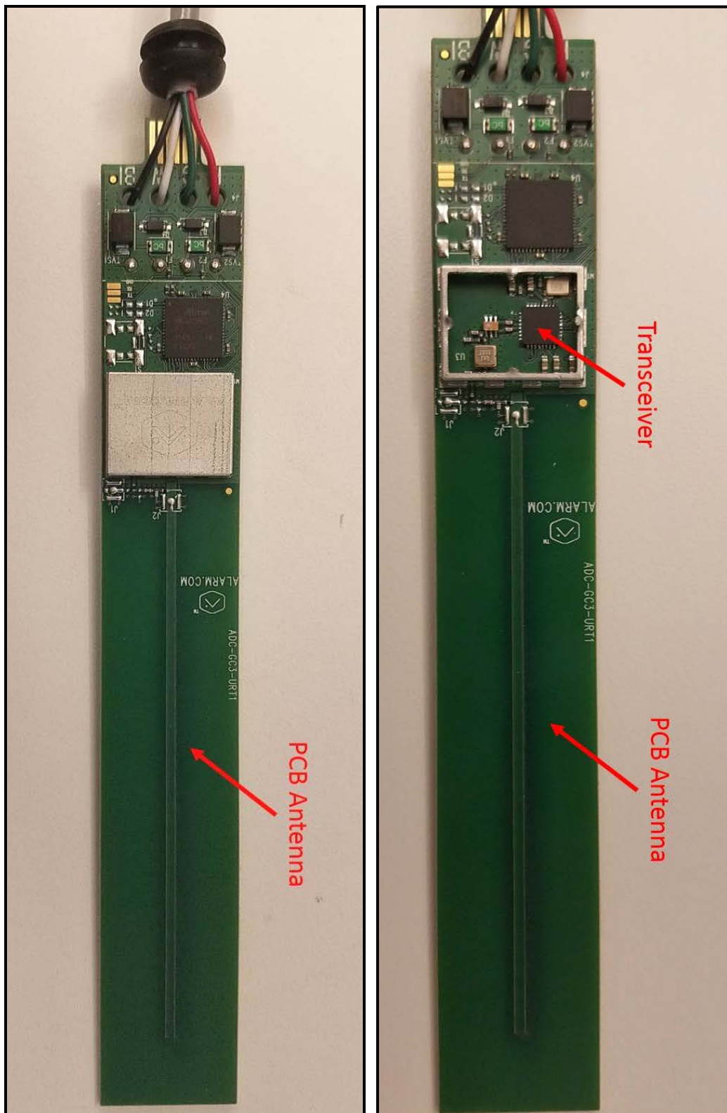
Photograph 7: Top View with Shield and without Shield
