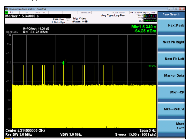
Radar Type 5 Calibration Plot
