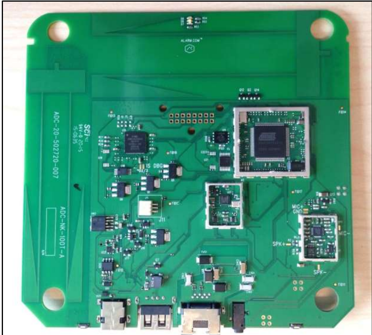
Photograph 21: Fully Populated PCB – Bottom View without Shields
