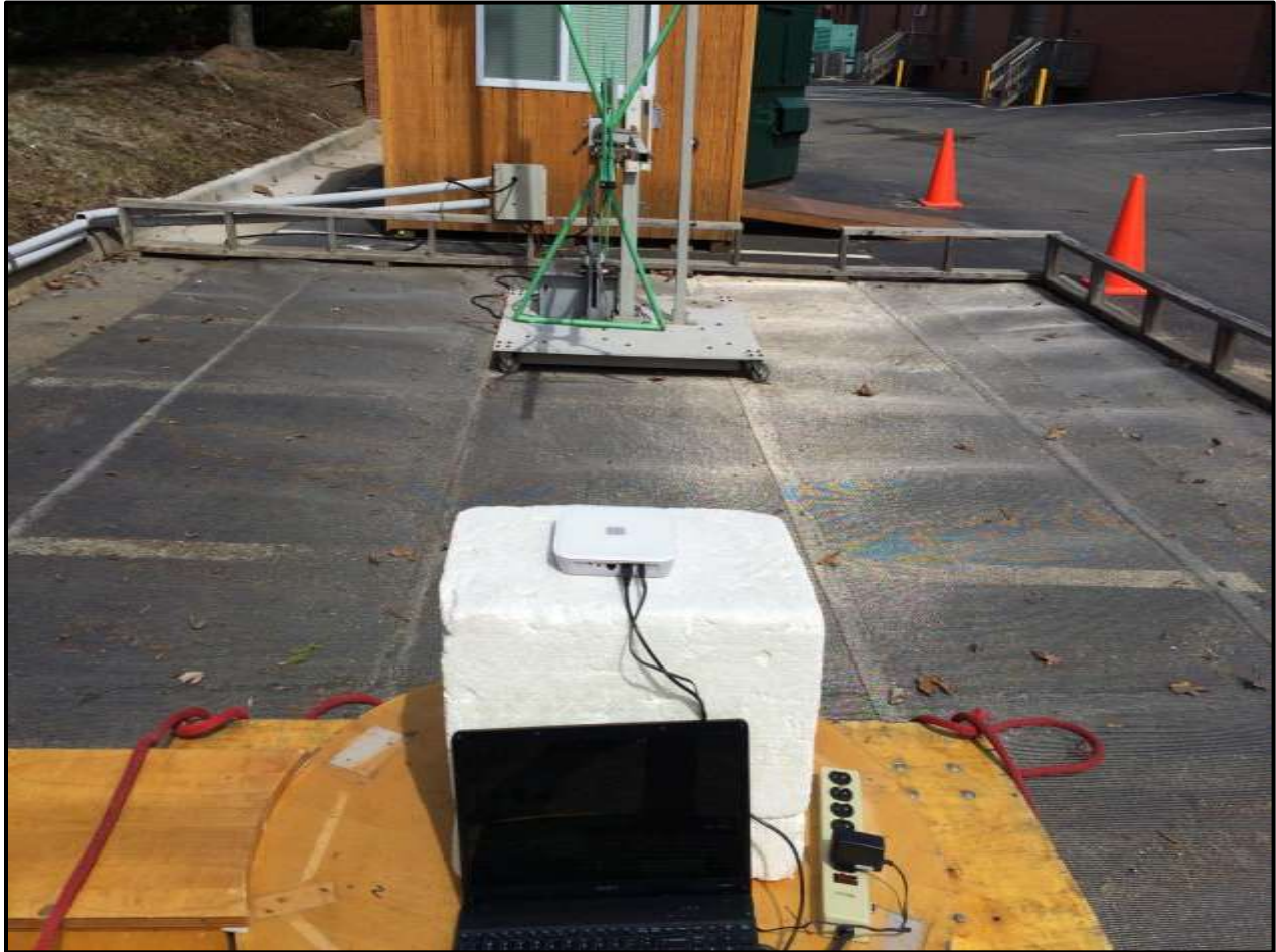
Photograph 2: Radiated Emissions Testing – Back View
