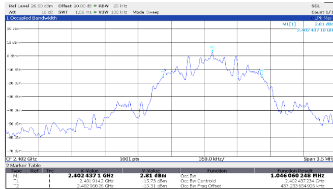
Figure 8.8-1: 99% occupied bandwidth, GFSK, 0.125 Mbps, 2402 MHz
