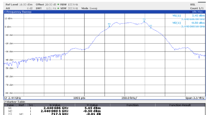
Figure 8.4-8: Minimum 6 dB bandwidth, GFSK, 1 Mbps, 2440 MHz
