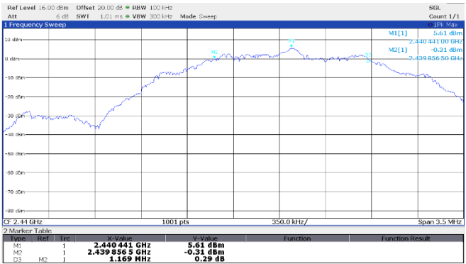
Figure 8.4-11: Minimum 6 dB bandwidth, GFSK, 2 Mbps, 2440 MHz
