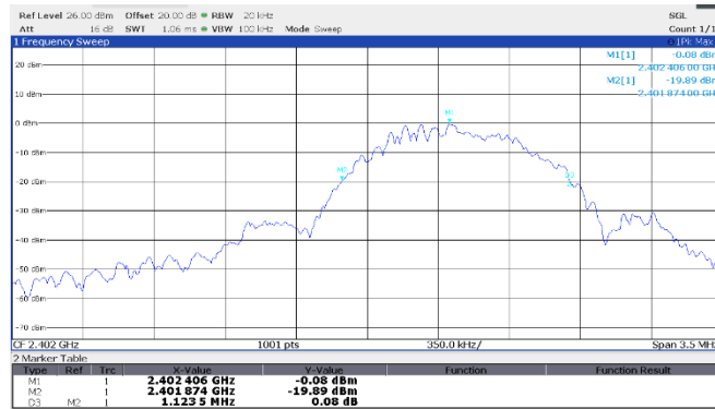
Figure 8.3-7: 20 dB bandwidth, GFSK, 1 Mbps, 2402 MHz
