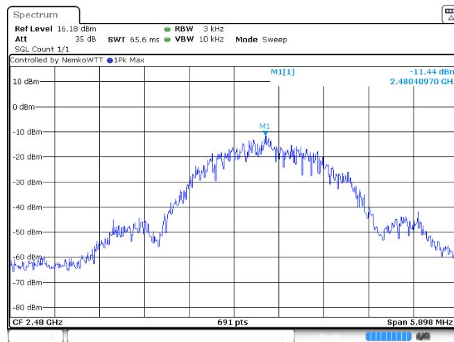
Peak power spectral density, TX 2480 MHz, BW 1 MHz, MOD: GF SK_2Mbps
