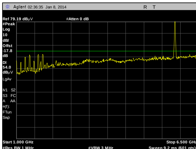
Plot 119. Radiated Spurious Emissions, Internal Antenna, 802.11n 20 MHz, 5785 MHz, 1 GHz – 6.5 GHz, Peak under Average
