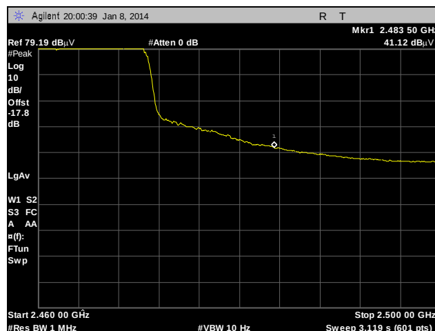
Plot 189. Radiated Restricted Band Edge, External Antenna, 802.11g, High Channel, Average
