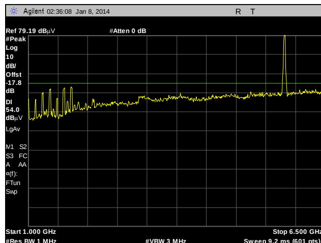
Plot 116. Radiated Spurious Emissions, Internal Antenna, 802.11n 20 MHz, 5745 MHz, 1 GHz – 6.5 GHz, Peak under Average
