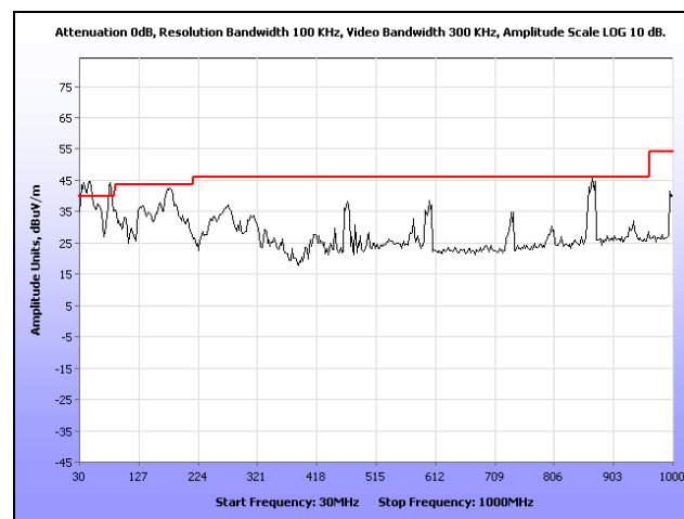
Plot 84. Radiated Spurious Emissions, External Antenna, 802.11g, 2412 MHz, 30 MHz – 1 GHz
