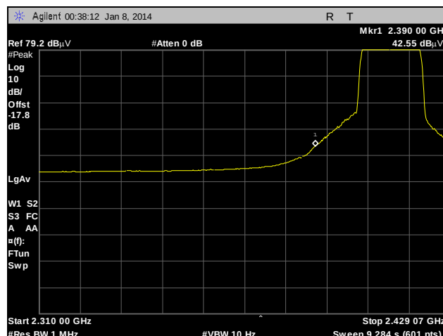
Plot 171. Radiated Restricted Band Edge, Internal Antenna, 802.11g, Low Channel, Average
