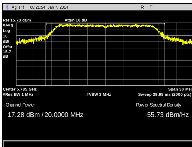
Plot 34. Peak Power Output, 802.11a, Mid Channel, 5785 MHz, Port B
