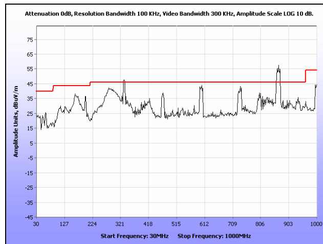
Plot 70. Radiated Spurious Emissions, Internal Antenna, 802.11n 40 MHz, 2422 MHz, 30 MHz – 1 GHz
