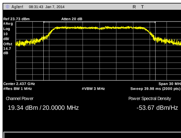
Plot 16. Peak Power Output, 802.11g, Mid Channel, 2437 MHz, Port B
