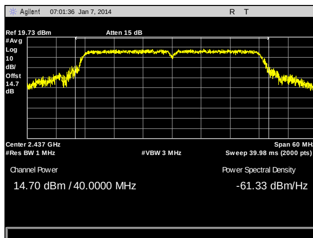
Plot 25. Peak Power Output, 802.11n 40 MHz, Mid Channel, 2437 MHz, Port A
