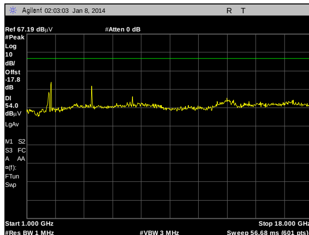
Plot 94. Radiated Spurious Emissions, External Antenna, 802.11n 20 MHz, 2437 MHz, 1 GHz – 18 GHz, Peak under Average
