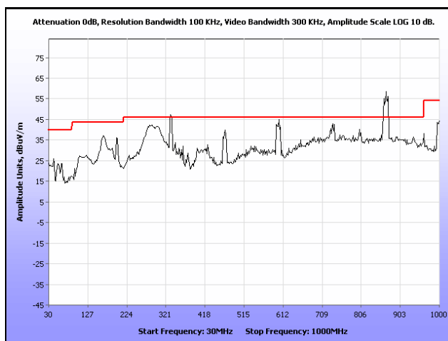
Plot 118. Radiated Spurious Emissions, Internal Antenna, 802.11n 20 MHz, 5785 MHz, 30 MHz – 1 GHz
