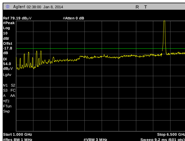
Plot 126. Radiated Spurious Emissions, Internal Antenna, 802.11n 40 MHz, 5755 MHz, 1 GHz – 6.5 GHz, Peak under Average
