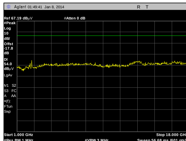
Plot 85. Radiated Spurious Emissions, External Antenna, 802.11g, 2412 MHz, 1 GHz – 18 GHz, Peak under Average
