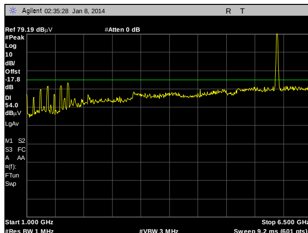
Plot 113. Radiated Spurious Emissions, Internal Antenna, 802.11a, 5825 MHz, 1 GHz – 6.5 GHz, Peak under Average
