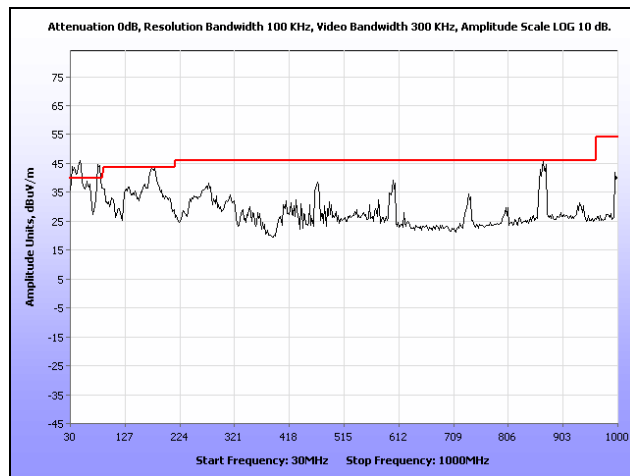
Plot 93. Radiated Spurious Emissions, External Antenna, 802.11n 20 MHz, 2437 MHz, 30 MHz – 1 GHz
