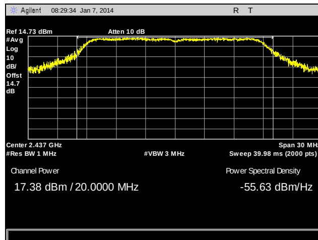
Plot 22. Peak Power Output, 802.11n 20 MHz, Mid Channel, 2437 MHz, Port B
