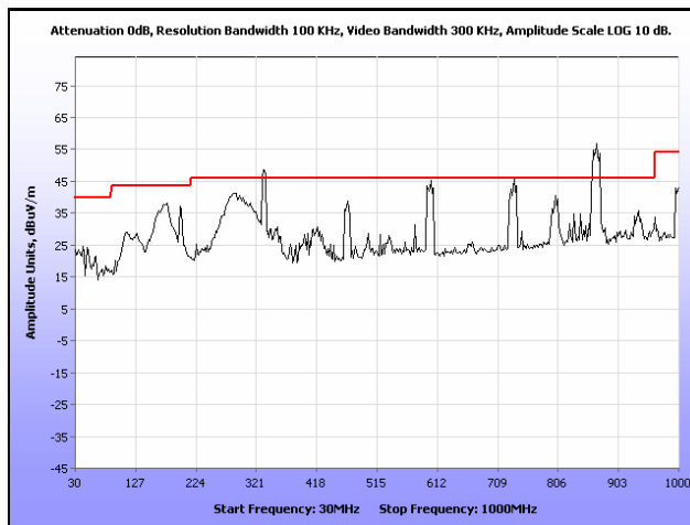
Plot 50. Radiated Spurious Emissions, Internal Antenna, 802.11b, 2437 MHz, 30 MHz – 1 GHz
