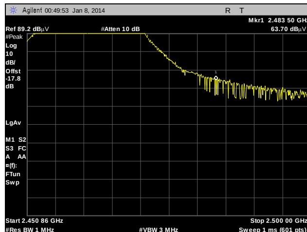
Plot 174. Radiated Restricted Band Edge, Internal Antenna, 802.11g, High Channel, Peak
