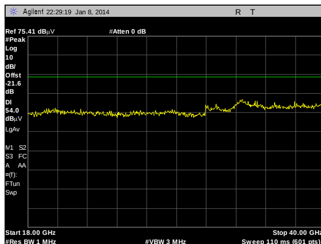
Plot 153. Radiated Spurious Emissions, External Antenna, 802.11n 20 MHz, 5785 MHz, 18 GHz – 40 GHz, Peak under Average
