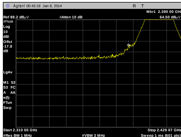
Plot 176. Radiated Restricted Band Edge, Internal Antenna, 802.11n 20 MHz, Low Channel, Peak
