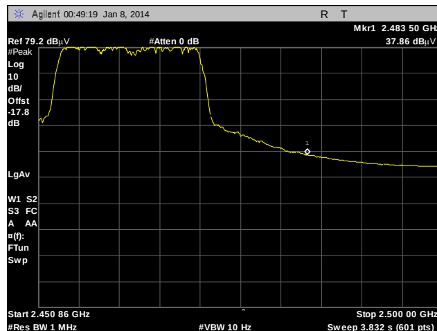
Plot 173. Radiated Restricted Band Edge, Internal Antenna, 802.11g, High Channel, Average
