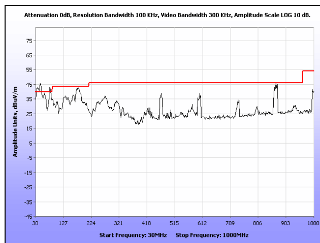
Plot 96. Radiated Spurious Emissions, External Antenna, 802.11n 20 MHz, 2462 MHz, 30 MHz – 1 GHz
