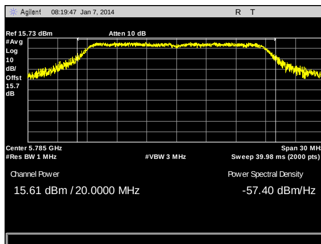
Plot 40. Peak Power Output, 802.11n 20 MHz, Mid Channel, 5785 MHz, Port B
