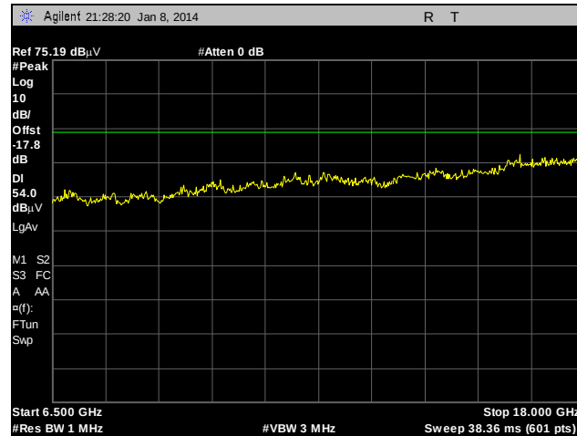
Plot 165. Radiated Spurious Emissions, External Antenna, 802.11n 40 MHz, 5795 MHz, 6.5 GHz – 18 GHz, Peak under Average
