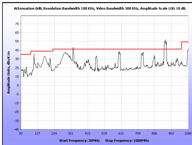
Plot 65. Radiated Spurious Emissions, Internal Antenna, 802.11n 20 MHz, 2437 MHz, 30 MHz – 1 GHz
