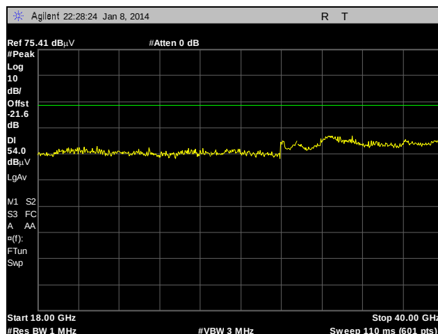
Plot 140. Radiated Spurious Emissions, External Antenna, 802.11a, 5785 MHz, 18 GHz – 40 GHz, Peak under Average
