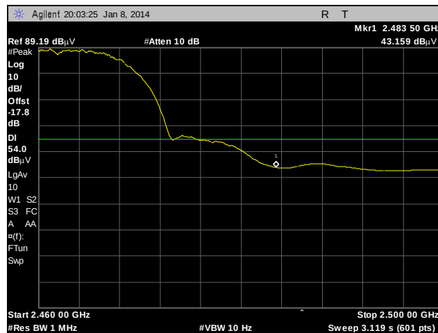
Plot 185. Radiated Restricted Band Edge, External Antenna, 802.11b, High Channel, Average
