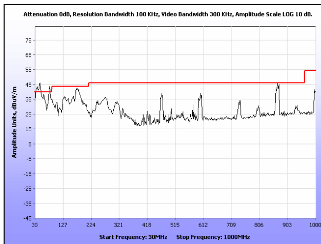
Plot 79. Radiated Spurious Emissions, External Antenna, 802.11b, 2437 MHz, 30 MHz – 1 GHz
