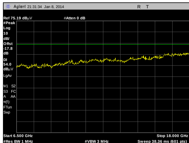
Plot 152. Radiated Spurious Emissions, External Antenna, 802.11n 20 MHz, 5785 MHz, 6.5 GHz – 18 GHz, Peak under Average
