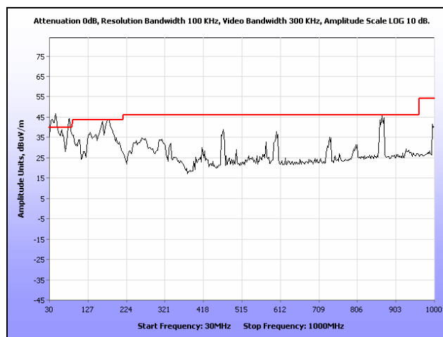
Plot 136. Radiated Spurious Emissions, External Antenna, 802.11a, 5785 MHz, 30 MHz – 1 GHz
