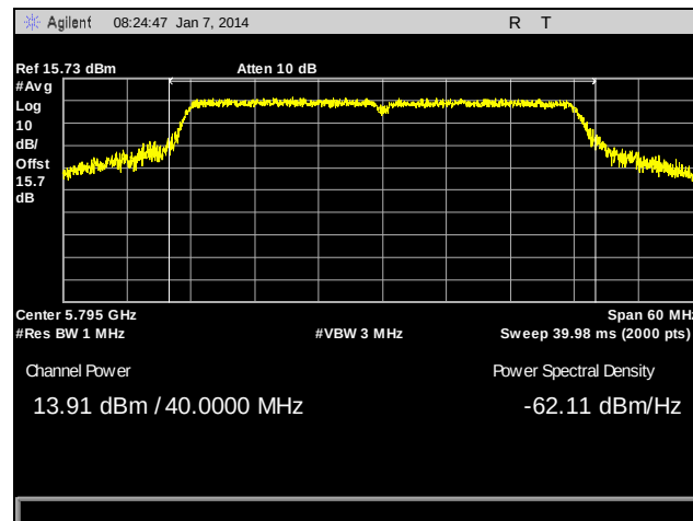
Plot 45. Peak Power Output, 802.11n 40 MHz, High Channel, 5795 MHz, Port B
