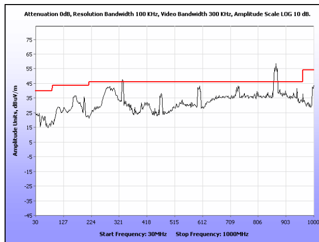
Plot 105. Radiated Spurious Emissions, Internal Antenna, 802.11a, 5745 MHz, 30 MHz – 1 GHz
