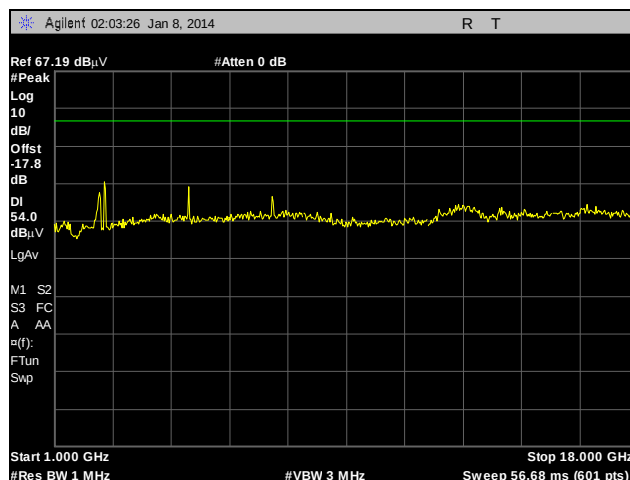
Plot 97. Radiated Spurious Emissions, External Antenna, 802.11n 20 MHz, 2462 MHz, 1 GHz – 18 GHz, Peak under Average
