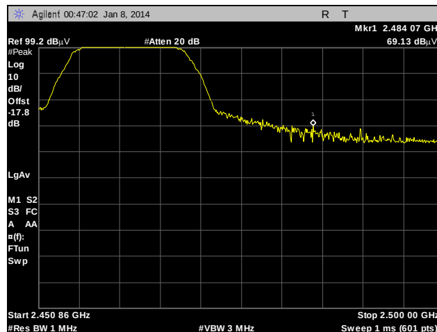
Plot 170. Radiated Restricted Band Edge, Internal Antenna, 802.11b, High Channel, Peak
