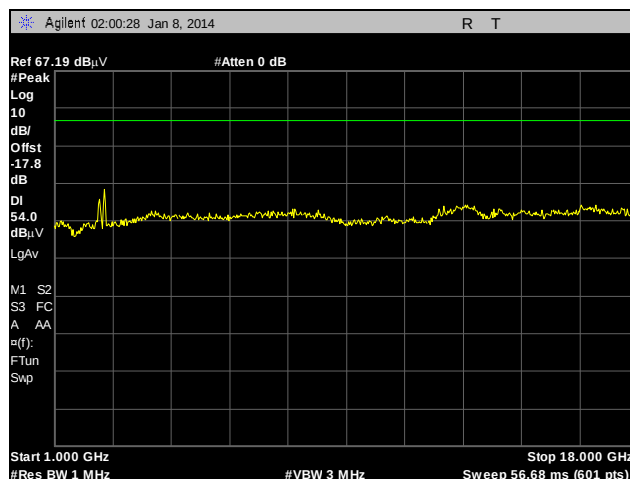
Plot 101. Radiated Spurious Emissions, External Antenna, 802.11n 40 MHz, 2437 MHz, 1 GHz – 18 GHz, Peak under Average
