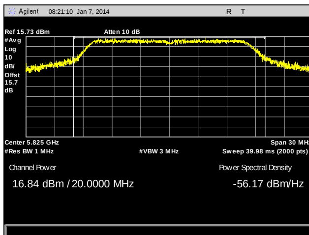
Plot 35. Peak Power Output, 802.11a, High Channel, 5825 MHz, Port B
