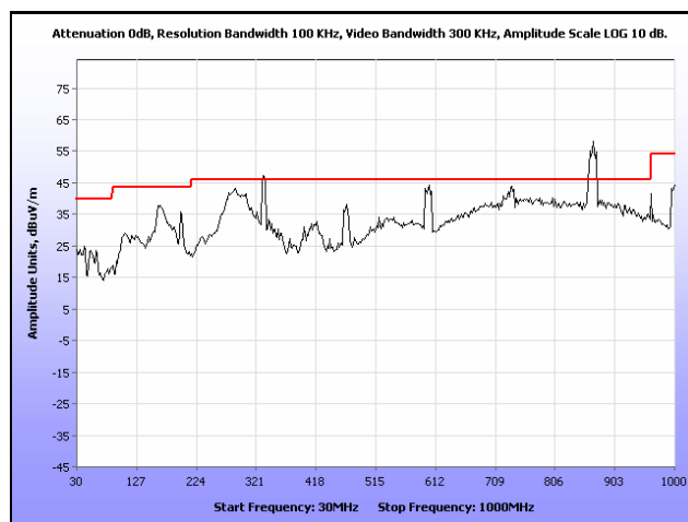
Plot 112. Radiated Spurious Emissions, Internal Antenna, 802.11a, 5825 MHz, 30 MHz – 1 GHz
