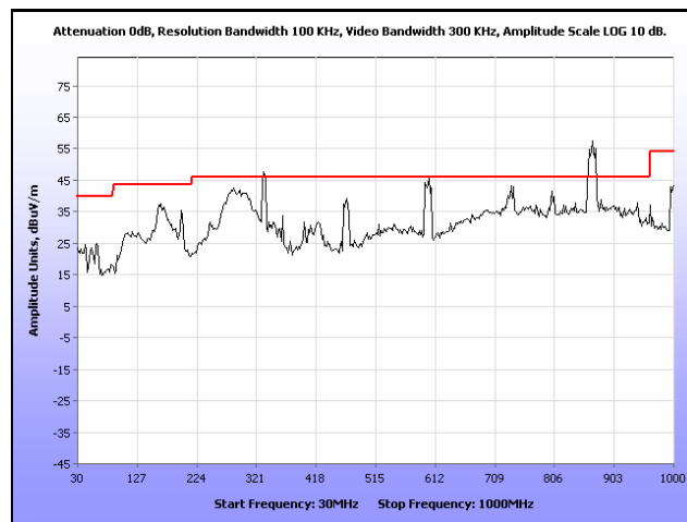
Plot 115. Radiated Spurious Emissions, Internal Antenna, 802.11n 20 MHz, 5745 MHz, 30 MHz – 1 GHz
