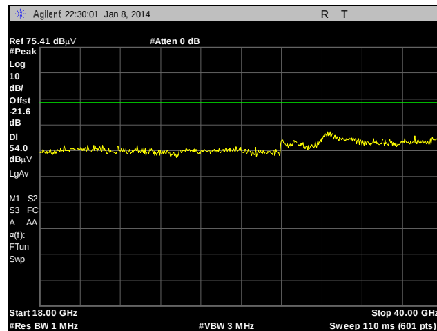
Plot 166. Radiated Spurious Emissions, External Antenna, 802.11n 40 MHz, 5795 MHz, 18 GHz – 40 GHz, Peak under Average
