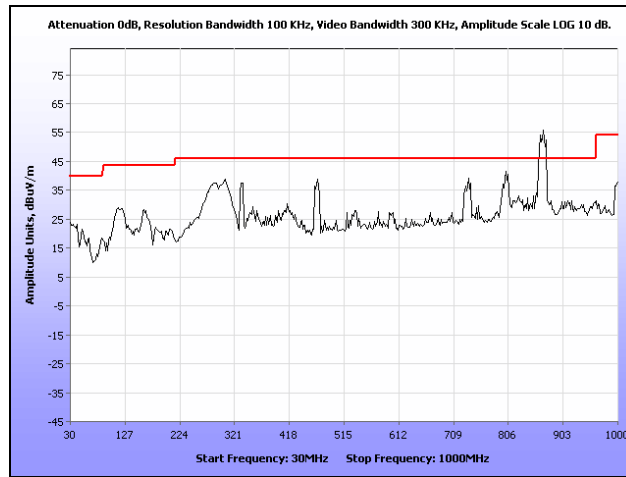
Plot 64. Radiated Spurious Emissions, Internal Antenna, 802.11a, 5240 MHz, 30 MHz – 1 GHz
