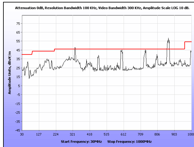
Plot 106. Radiated Spurious Emissions, Internal Antenna, 802.11a, 5500 MHz, 30 MHz – 1 GHz
