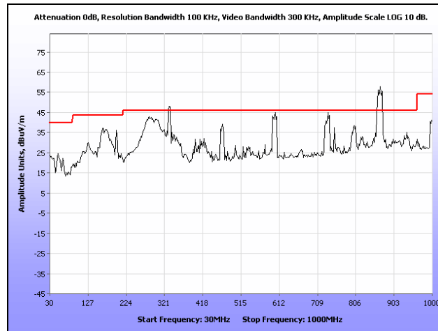
Plot 73. Radiated Spurious Emissions, Internal Antenna, 802.11n 20 MHz, 5240 MHz, 30 MHz – 1 GHz
