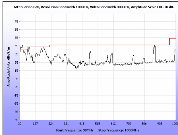
Plot 211. Radiated Spurious Emissions, External Antenna, 802.11n 40 MHz, 5670 MHz, 30 MHz – 1 GHz
