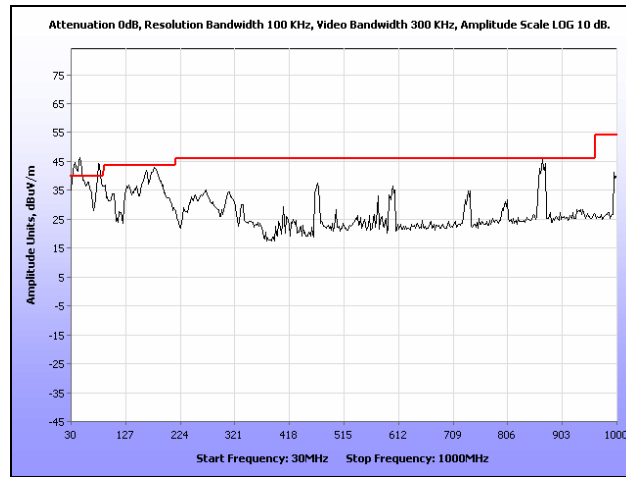
Plot 187. Radiated Spurious Emissions, External Antenna, 802.11a, 5580 MHz, 30 MHz – 1 GHz
