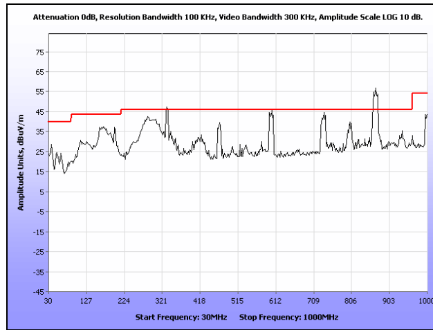
Plot 70. Radiated Spurious Emissions, Internal Antenna, 802.11n 20 MHz, 5200 MHz, 30 MHz – 1 GHz
