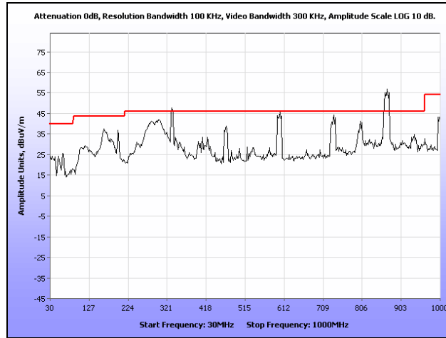
Plot 61. Radiated Spurious Emissions, Internal Antenna, 802.11a, 5200 MHz, 30 MHz – 1 GHz
