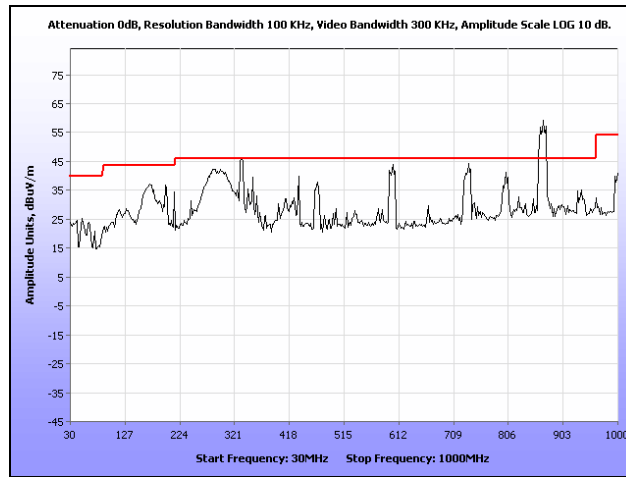
Plot 88. Radiated Spurious Emissions, Internal Antenna, 802.11a, 5320 MHz, 30 MHz – 1 GHz
