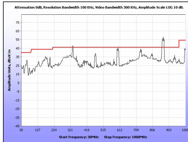
Plot 109. Radiated Spurious Emissions, Internal Antenna, 802.11a, 5580 MHz, 30 MHz – 1 GHz
