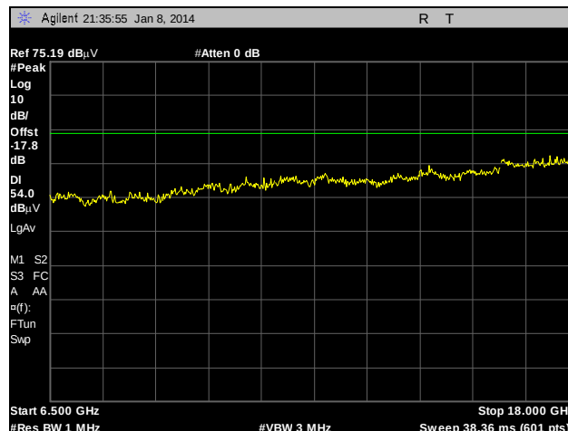
Plot 189. Radiated Spurious Emissions, External Antenna, 802.11a, 5580 MHz, 6.5 GHz – 18 GHz, Peak under Average
