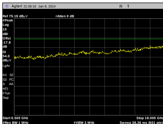
Plot 125. Radiated Spurious Emissions, Internal Antenna, 802.11n 20 MHz, 5700 MHz, 6.5 GHz – 18 GHz, Peak under Average
