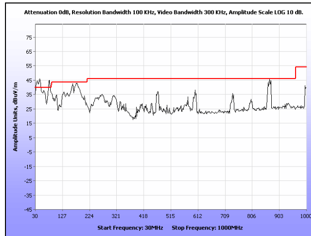
Plot 154. Radiated Spurious Emissions, External Antenna, 802.11n 40 MHz, 5190 MHz, 30 MHz – 1 GHz
