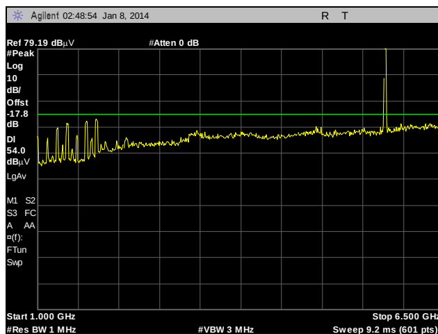
Plot 124. Radiated Spurious Emissions, Internal Antenna, 802.11n 20 MHz, 5700 MHz, 1 GHz – 6.5 GHz, Peak under Average
