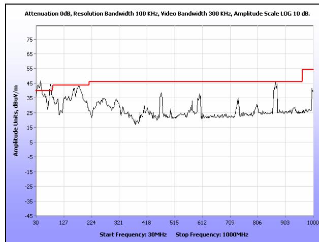
Plot 191. Radiated Spurious Emissions, External Antenna, 802.11a, 5700 MHz, 30 MHz – 1 GHz
