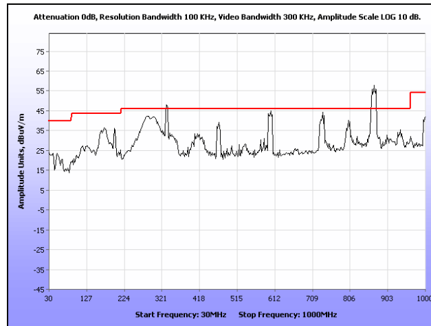
Plot 79. Radiated Spurious Emissions, Internal Antenna, 802.11n 40 MHz, 5230 MHz, 30 MHz – 1 GHz
