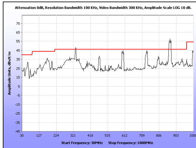
Plot 103. Radiated Spurious Emissions, Internal Antenna, 802.11n 40 MHz, 5310 MHz, 30 MHz – 1 GHz
