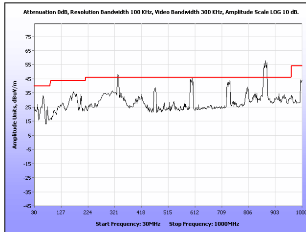
Plot 97. Radiated Spurious Emissions, Internal Antenna, 802.11n 20 MHz, 5320 MHz, 30 MHz – 1 GHz
