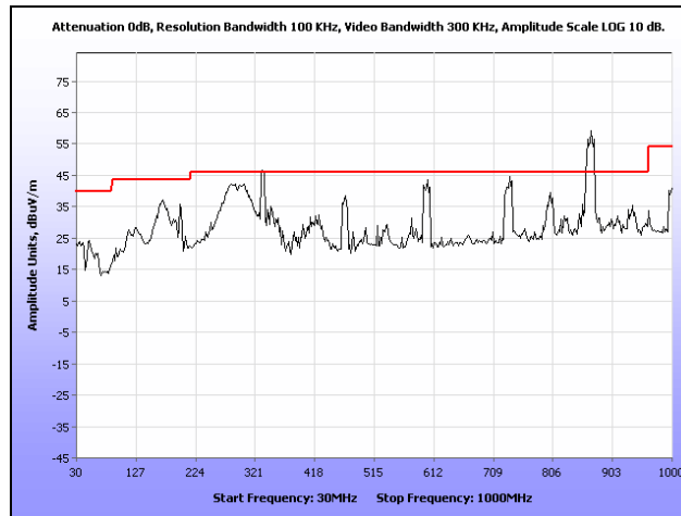
Plot 85. Radiated Spurious Emissions, Internal Antenna, 802.11a, 5300 MHz, 30 MHz – 1 GHz
