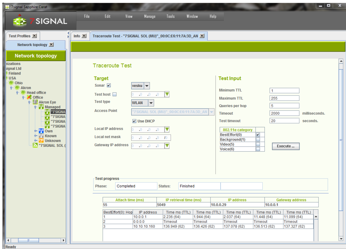
Figure 51: Traceroute test
