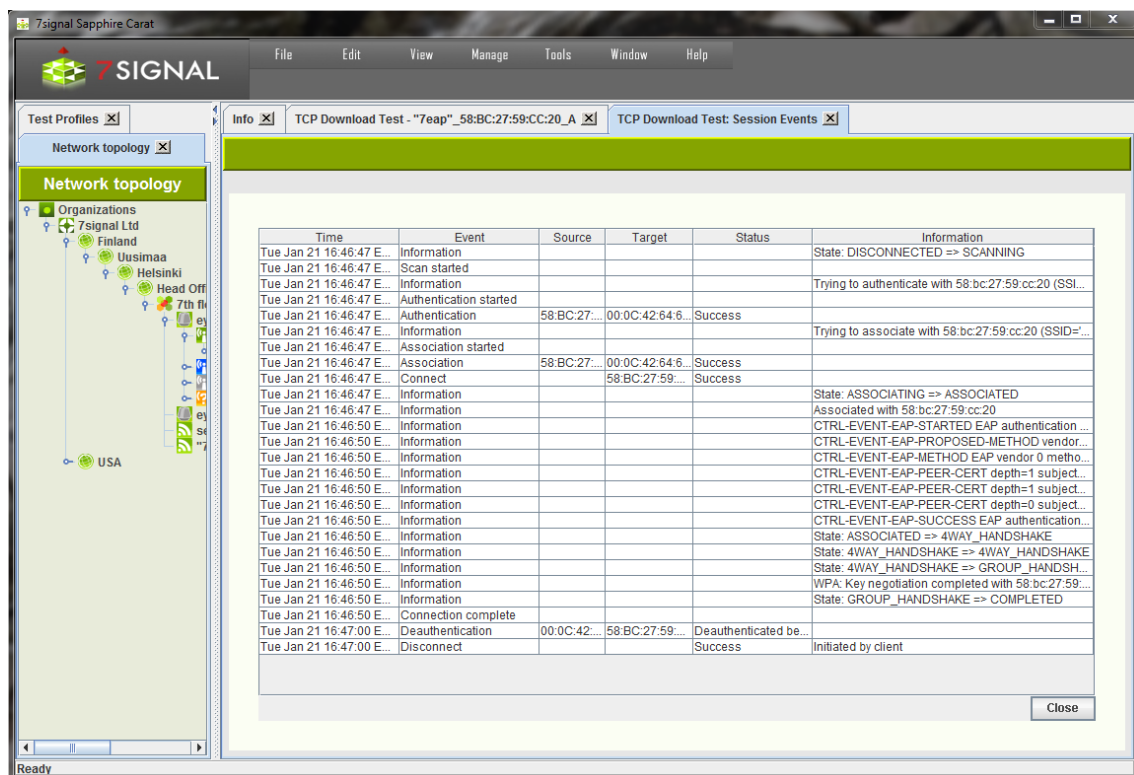
Figure 36: Session events
