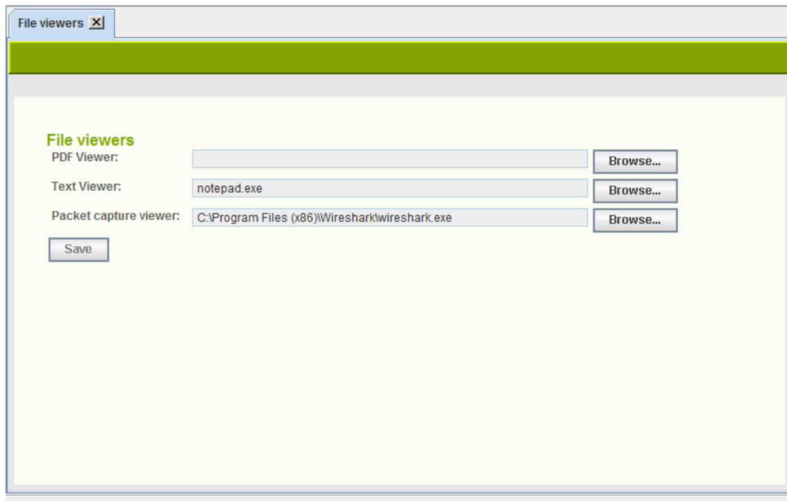
Figure 78: File viewer configuration
