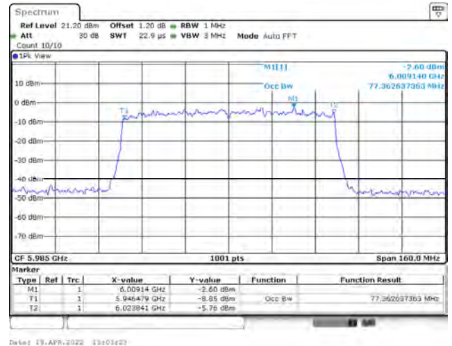
802.11ax (80MHz) / Ant. 2 / 5985 MHz (U-NII-5)
